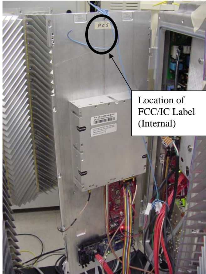
FlexWave™ URH – AWS Remote Unit Location of FCC/IC ID (Internal)
