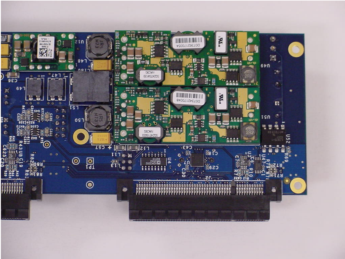
FlexWave™ URH RDI Bottom View - 2
