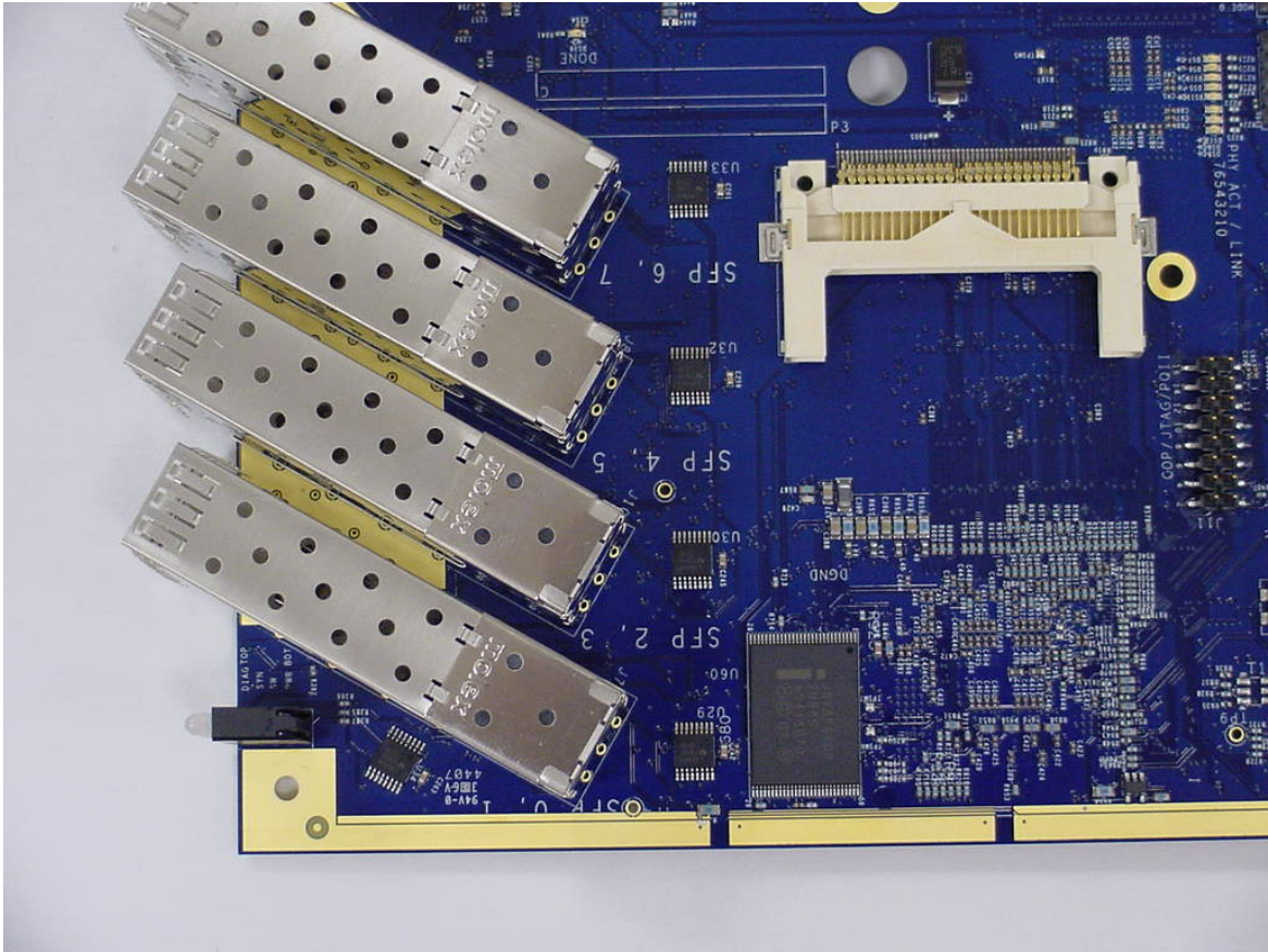
FlexWave™ URH SERF Top View – 1
