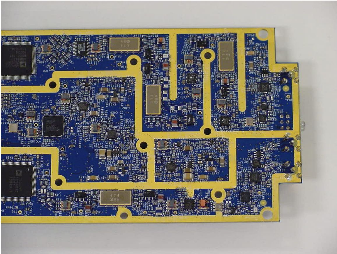
FlexWave™ URH DART Bottom View - 2
