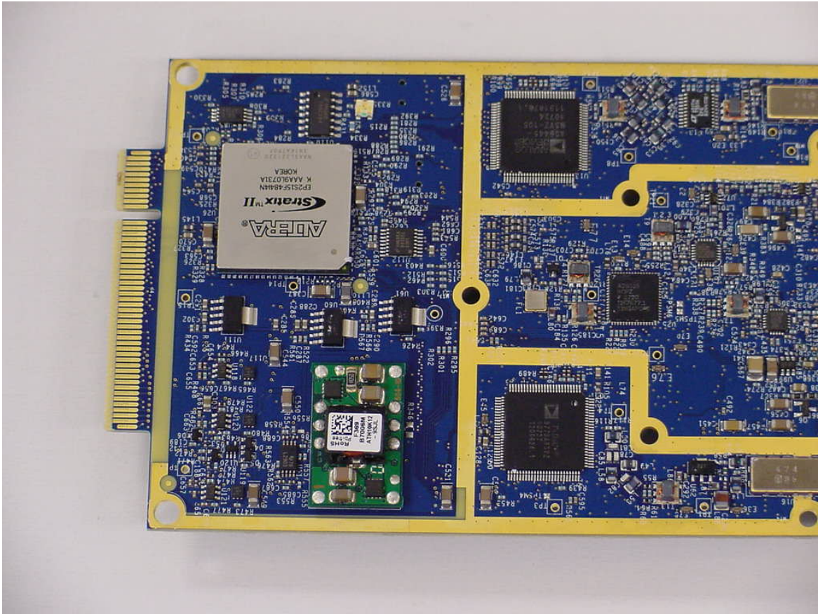
FlexWave™ URH DART Bottom View - 1
