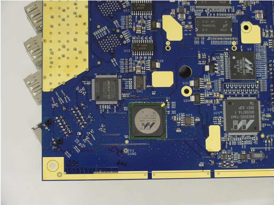
FlexWave™ URH SERF Bottom View - 1
