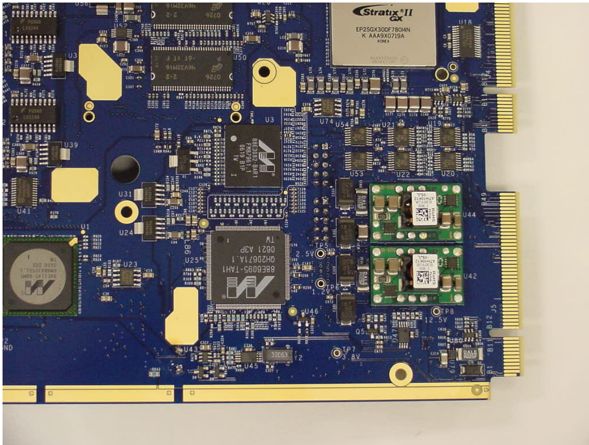
FlexWave™ URH SERF Bottom View - 2
