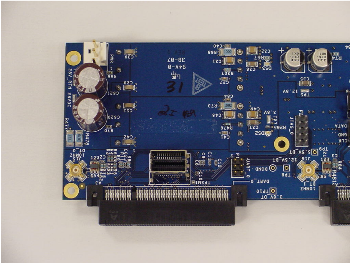
FlexWave™ URH RDI Top View – 1
