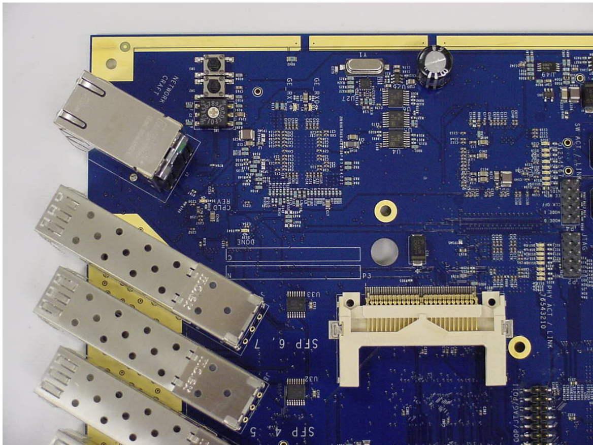
FlexWave™ URH SERF Top View - 4
