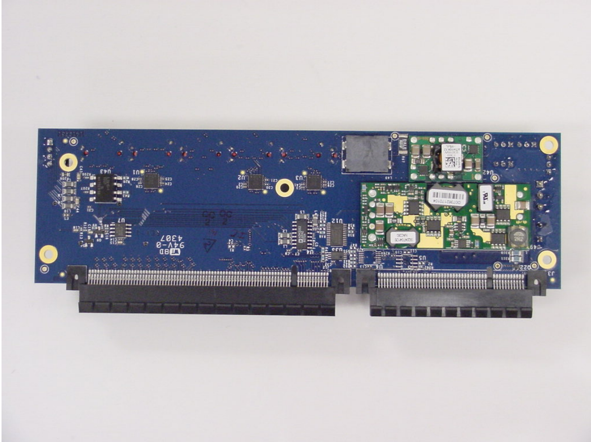
FlexWave™ URH RSI Top View
