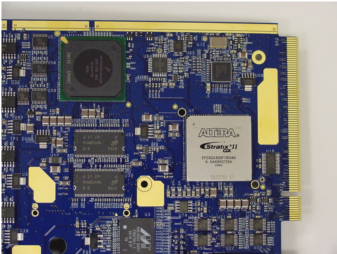
FlexWave™ URH SERF Bottom View – 3
