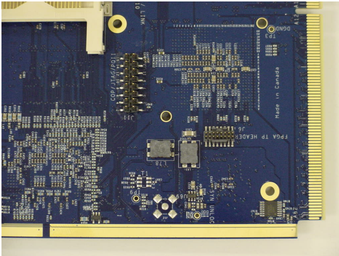
FlexWave™ URH SERF Top View - 2
