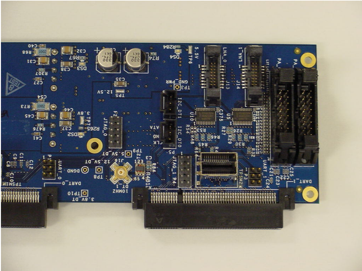
FlexWave™ URH RDI Top View - 2
