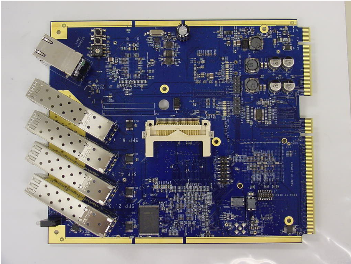
FlexWave™ URH SERF Top View
