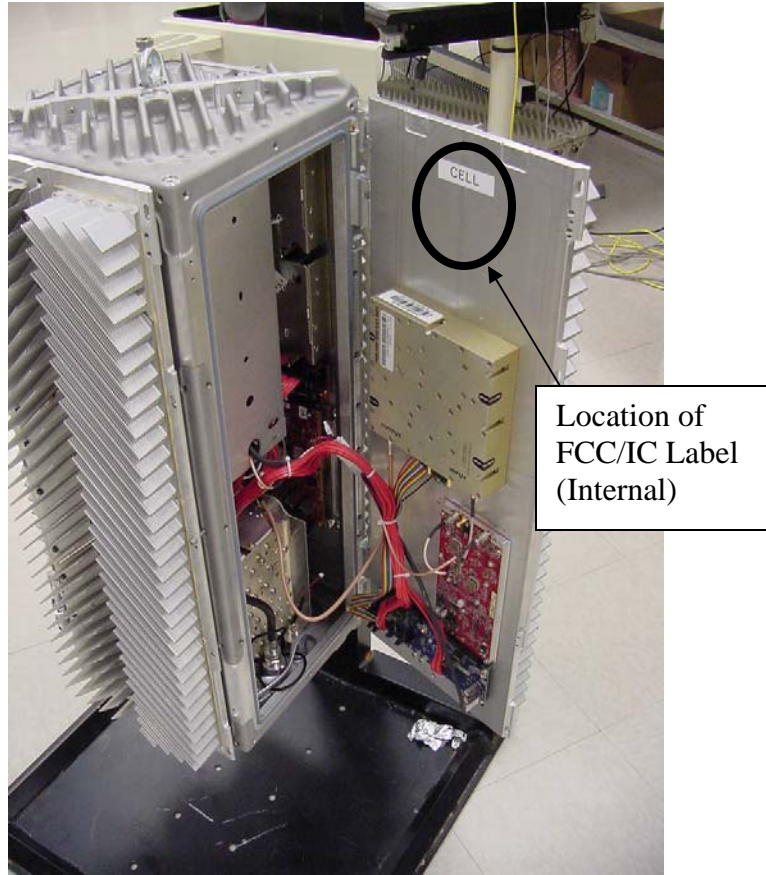
FlexWave™ URH - Cellular Remote Unit Location of FCC/IC ID (Internal)
