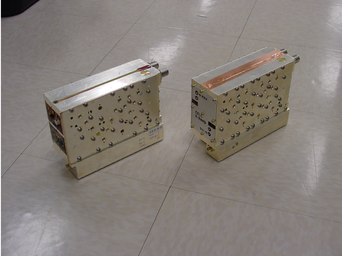
FlexWave™ URH Duplexer - Cellular Right View
