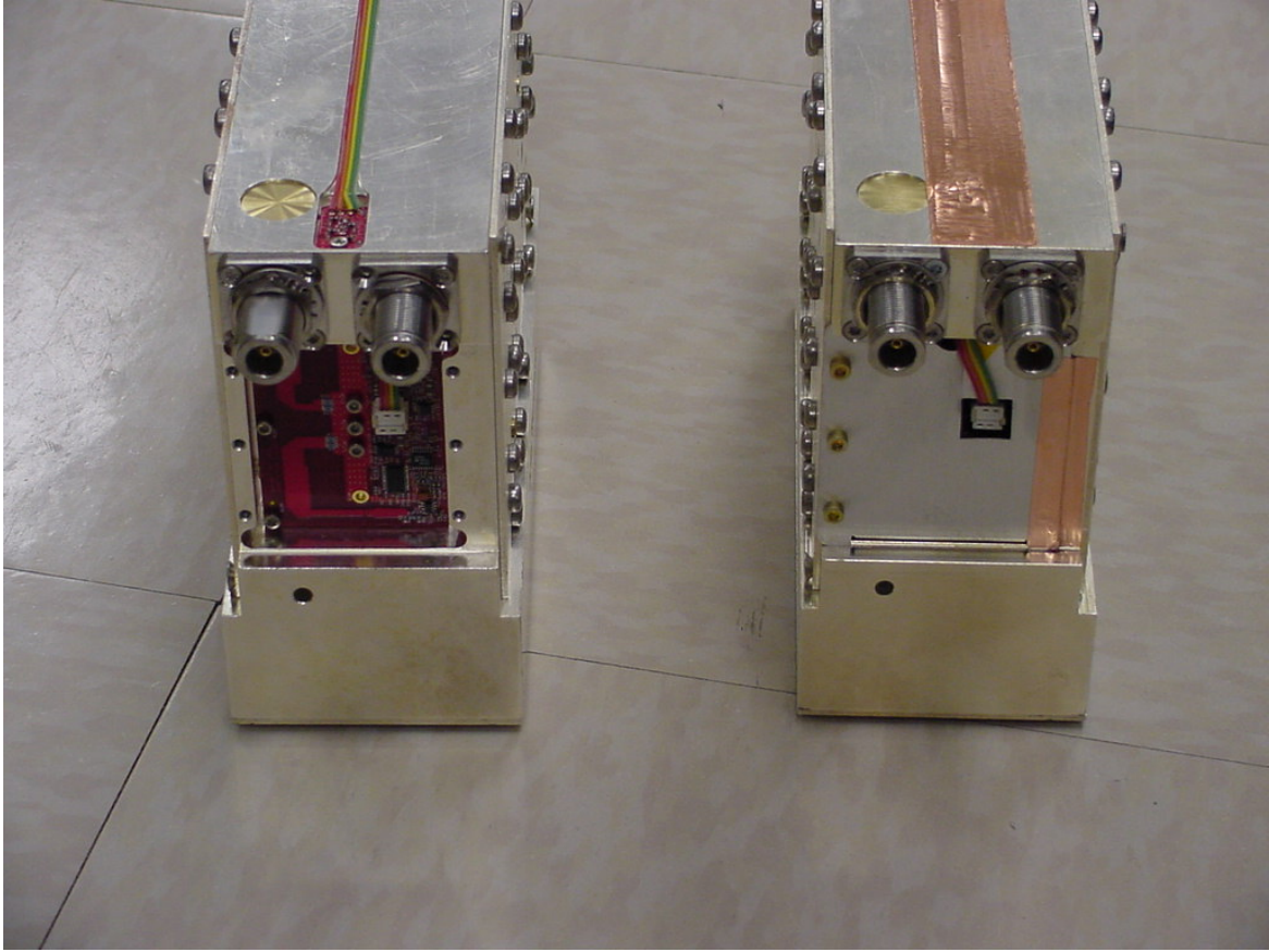
FlexWave™ URH Duplexer - Cellular Rear View
