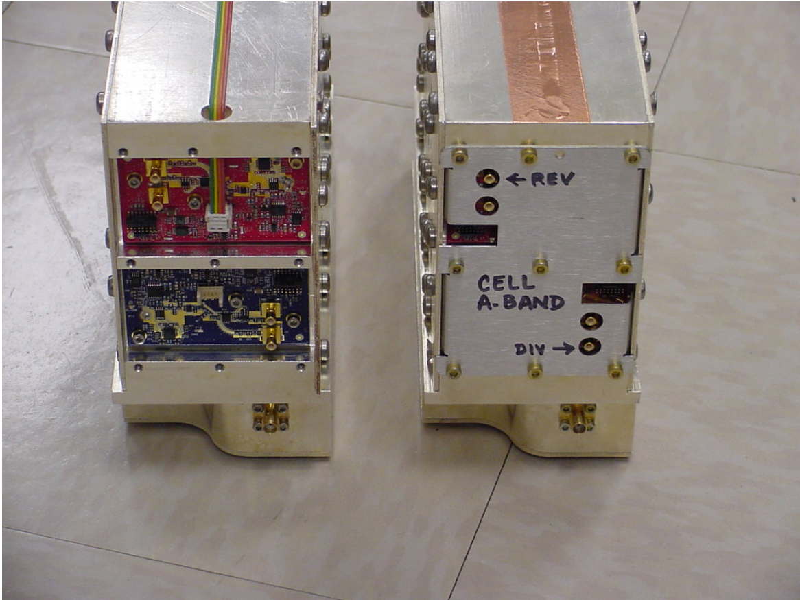
FlexWave™ URH Duplexer - Cellular Front View
