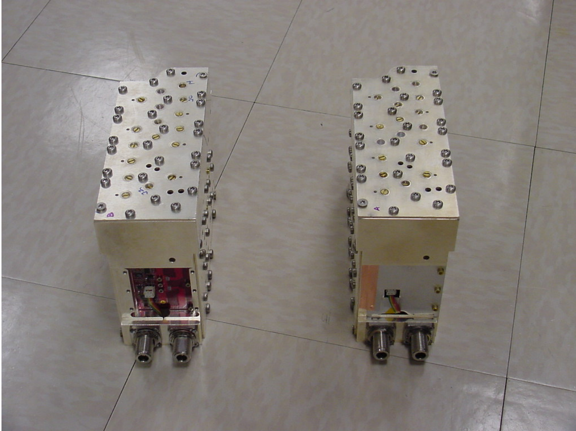
FlexWave™ URH Duplexer - Cellular Bottom View
