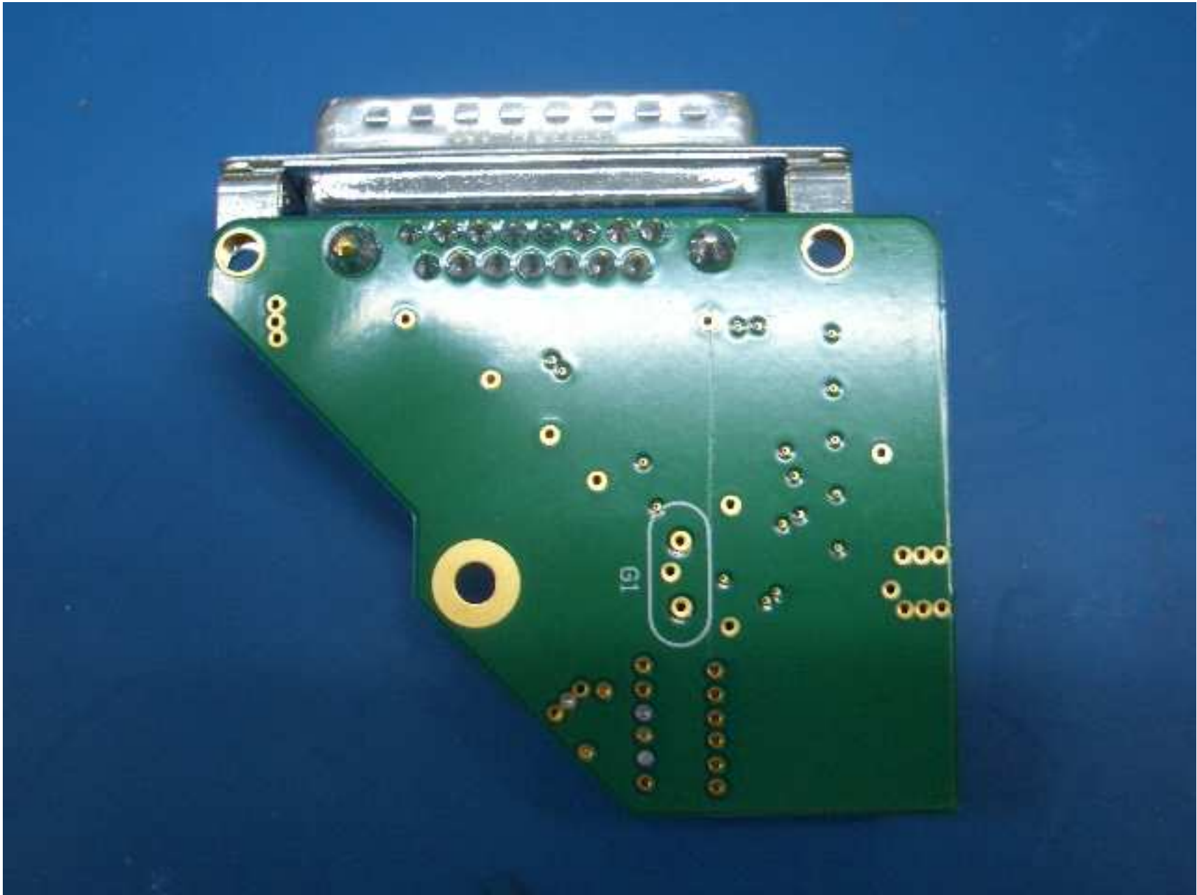
Power interface board back
