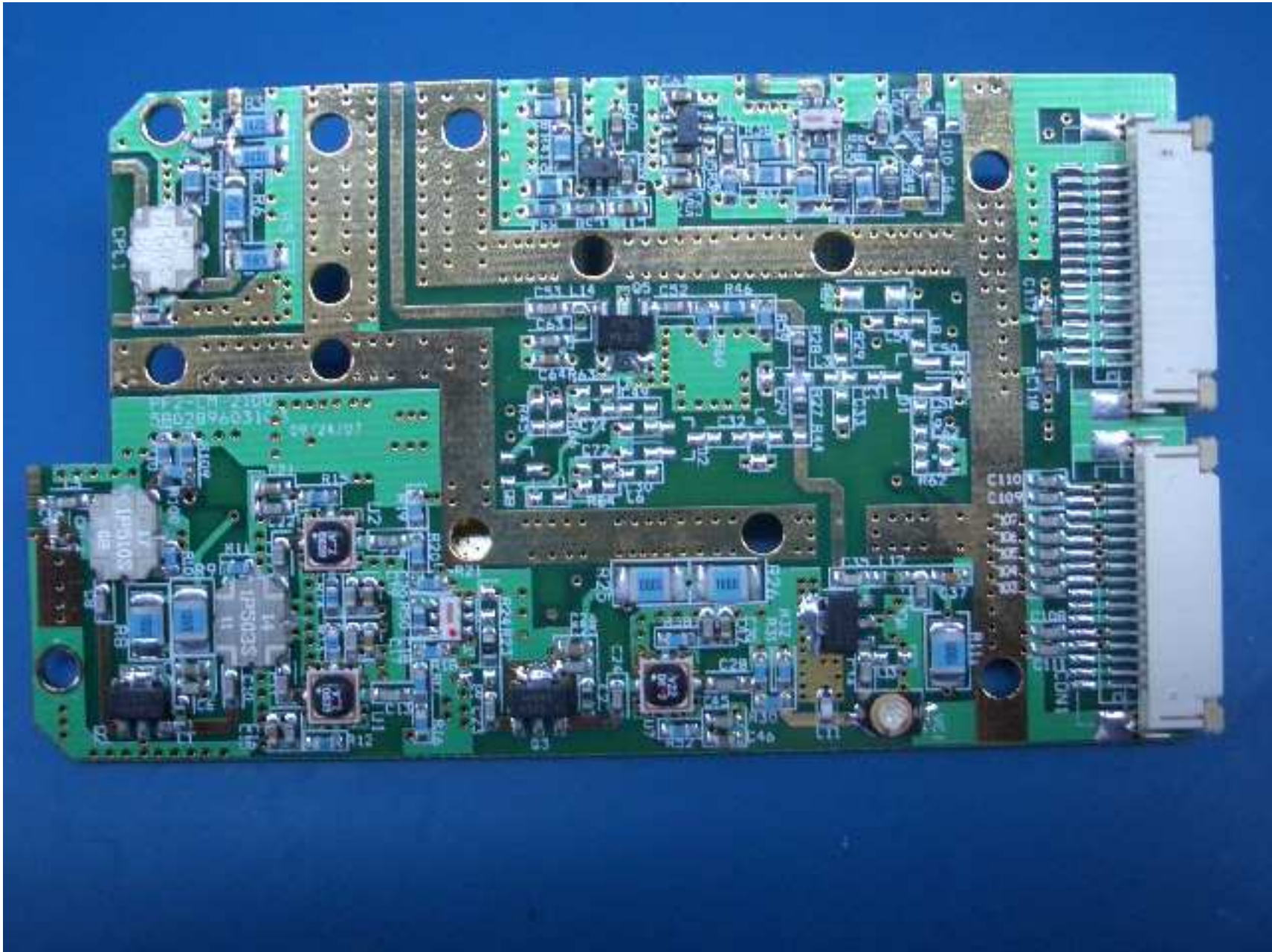
Main board back
