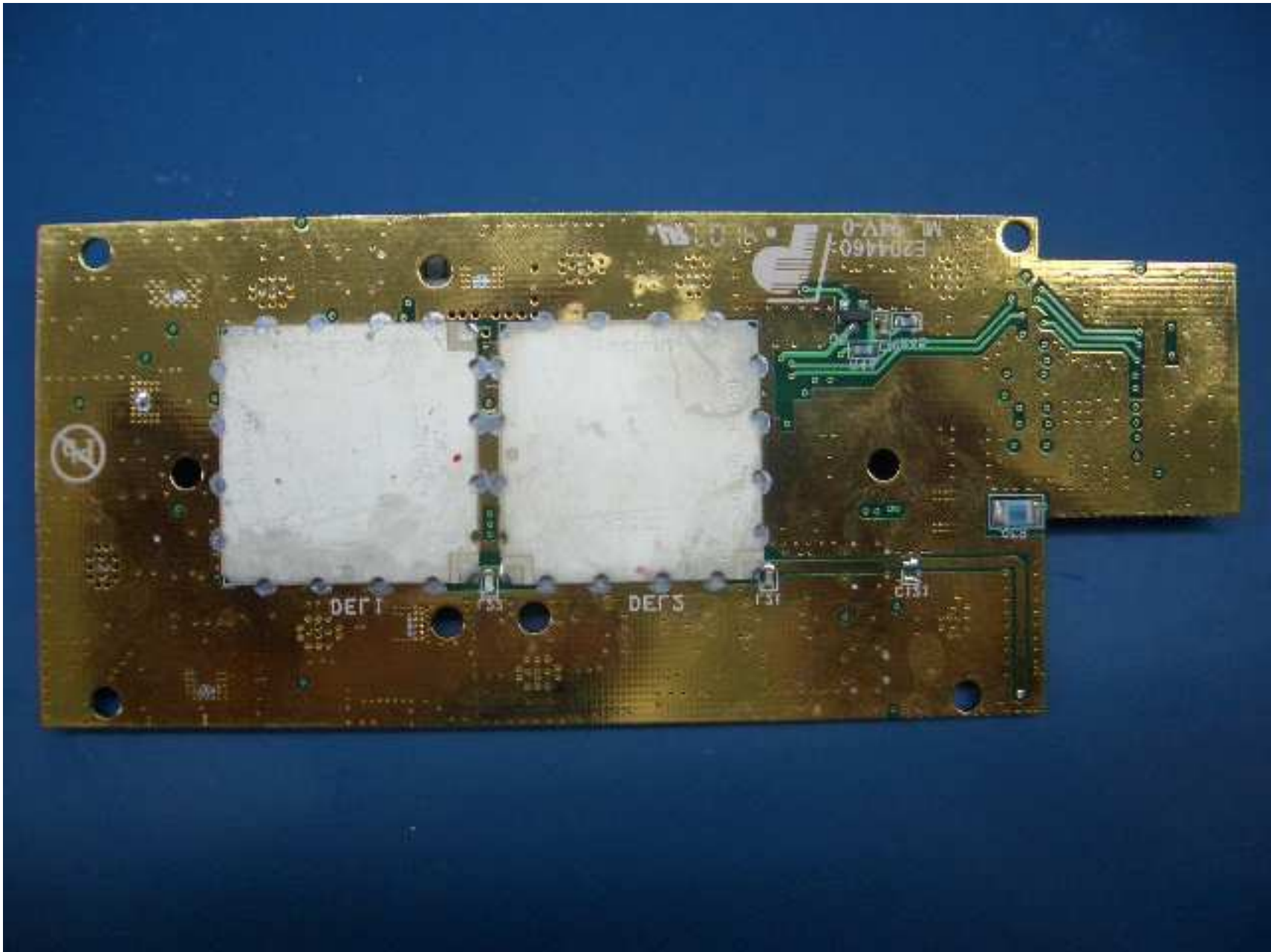
SSM board back
