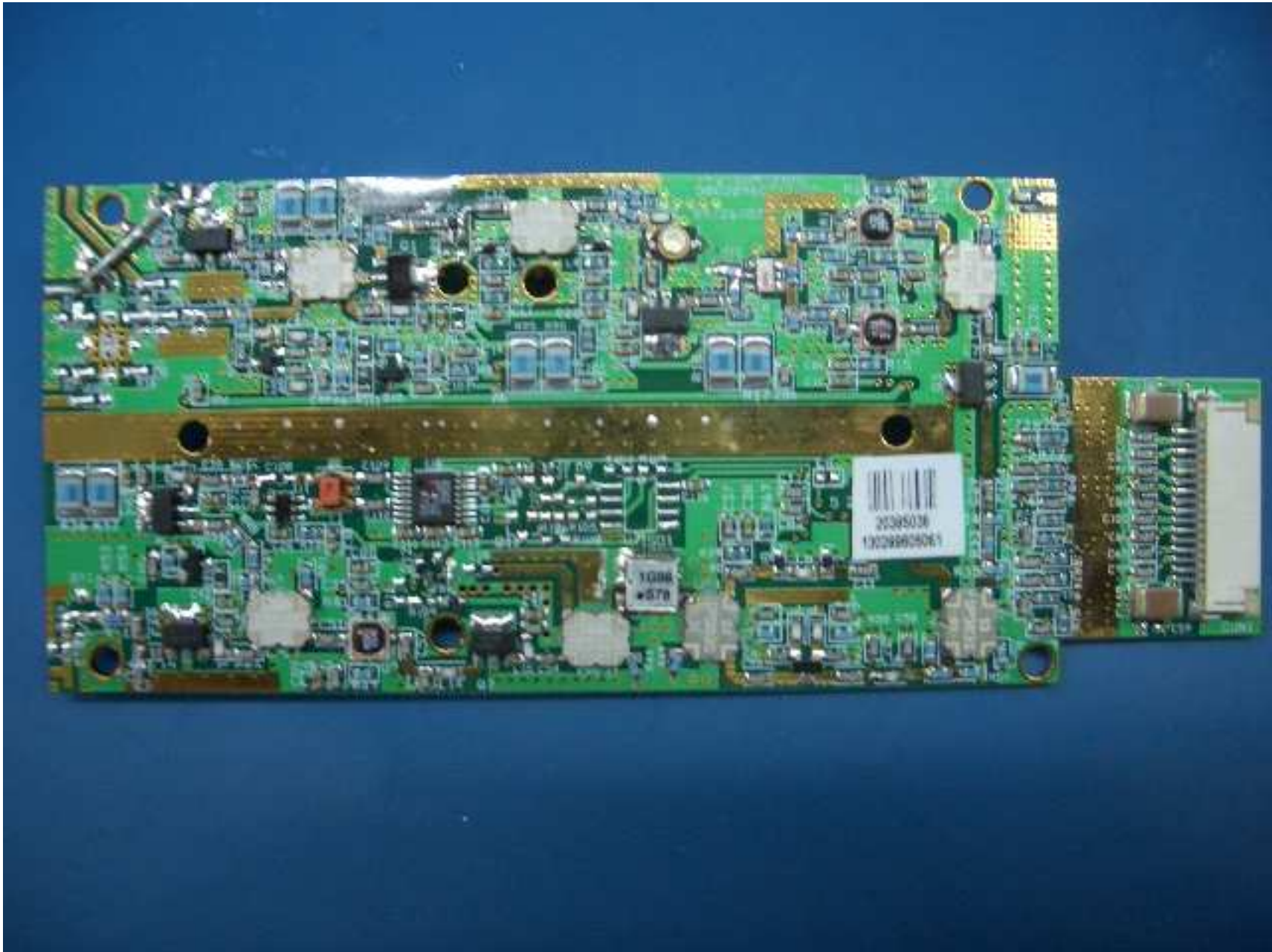
SSM board front
