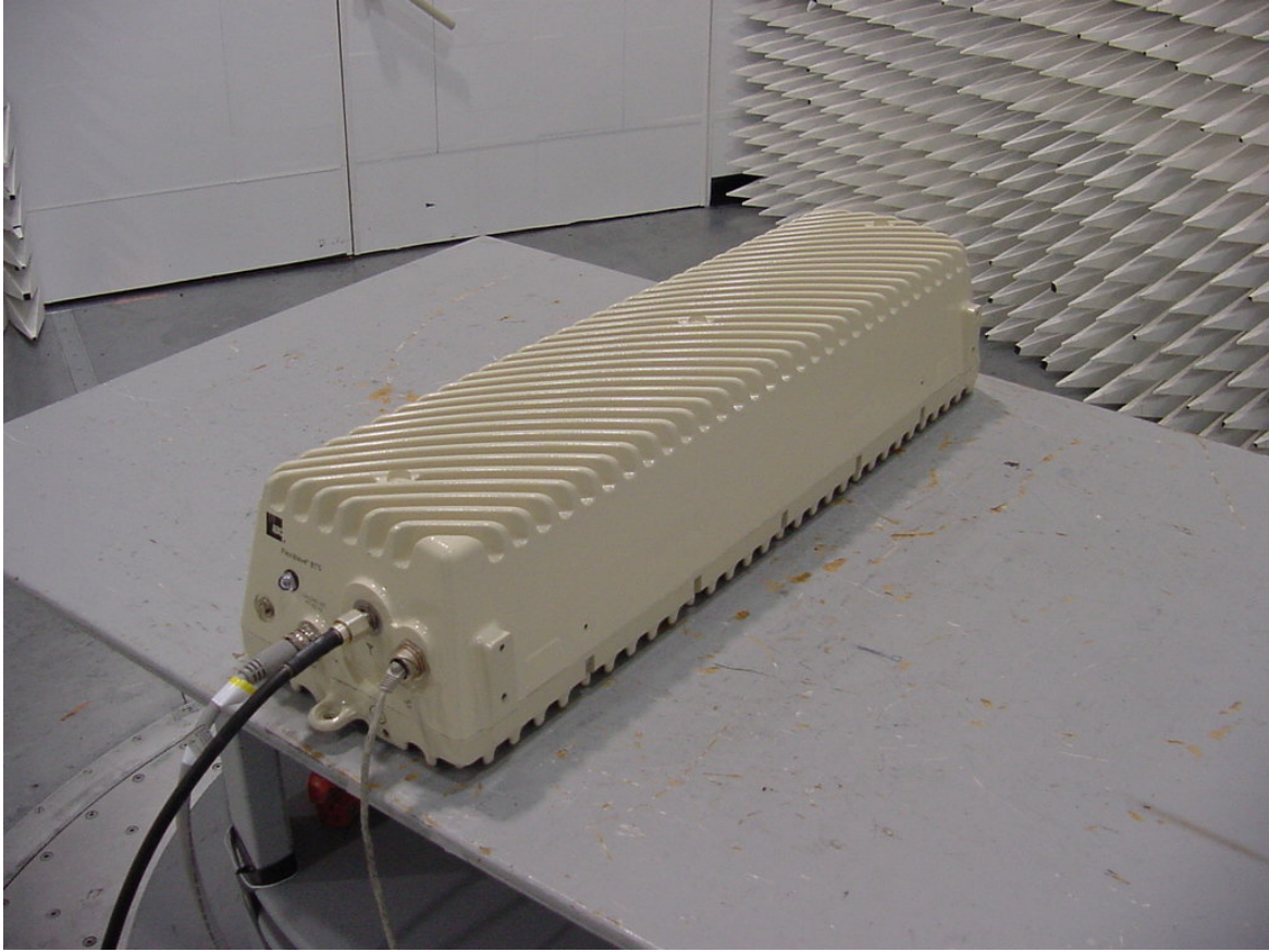
FlexWave™ microBTS Right View
