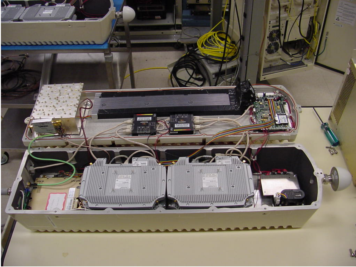
FlexWave™ microBTS Open View
