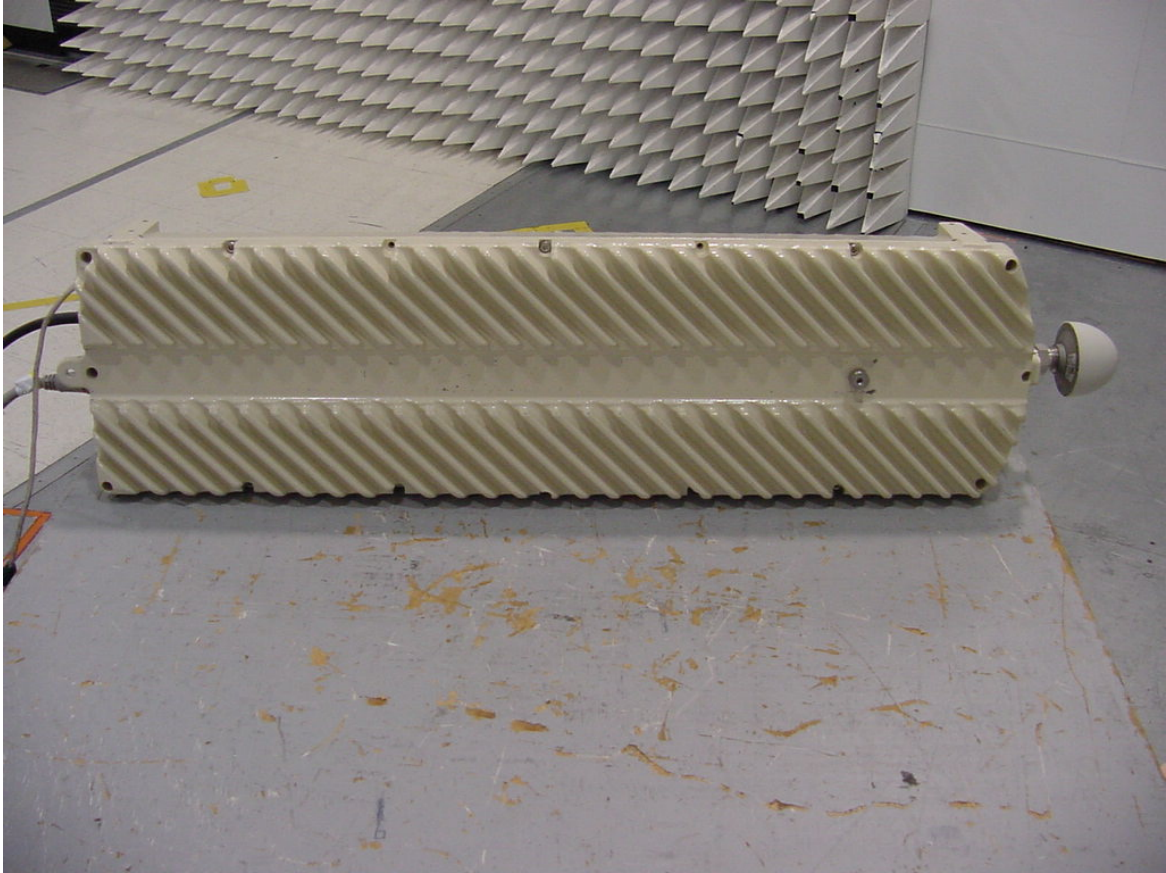
FlexWave™ microBTS Bottom View
