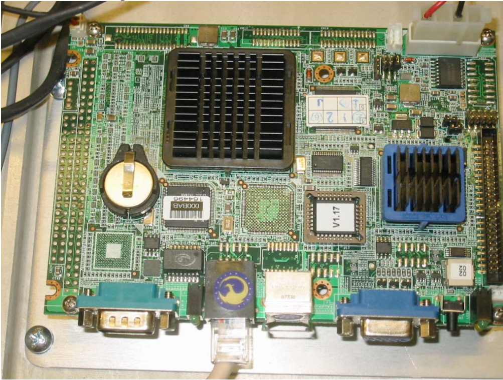
Processor board back
