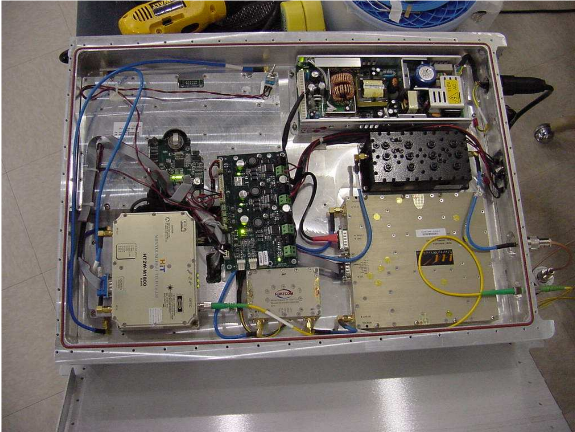
Digivance® WIMAX Remote Remote Unit Open Top View
