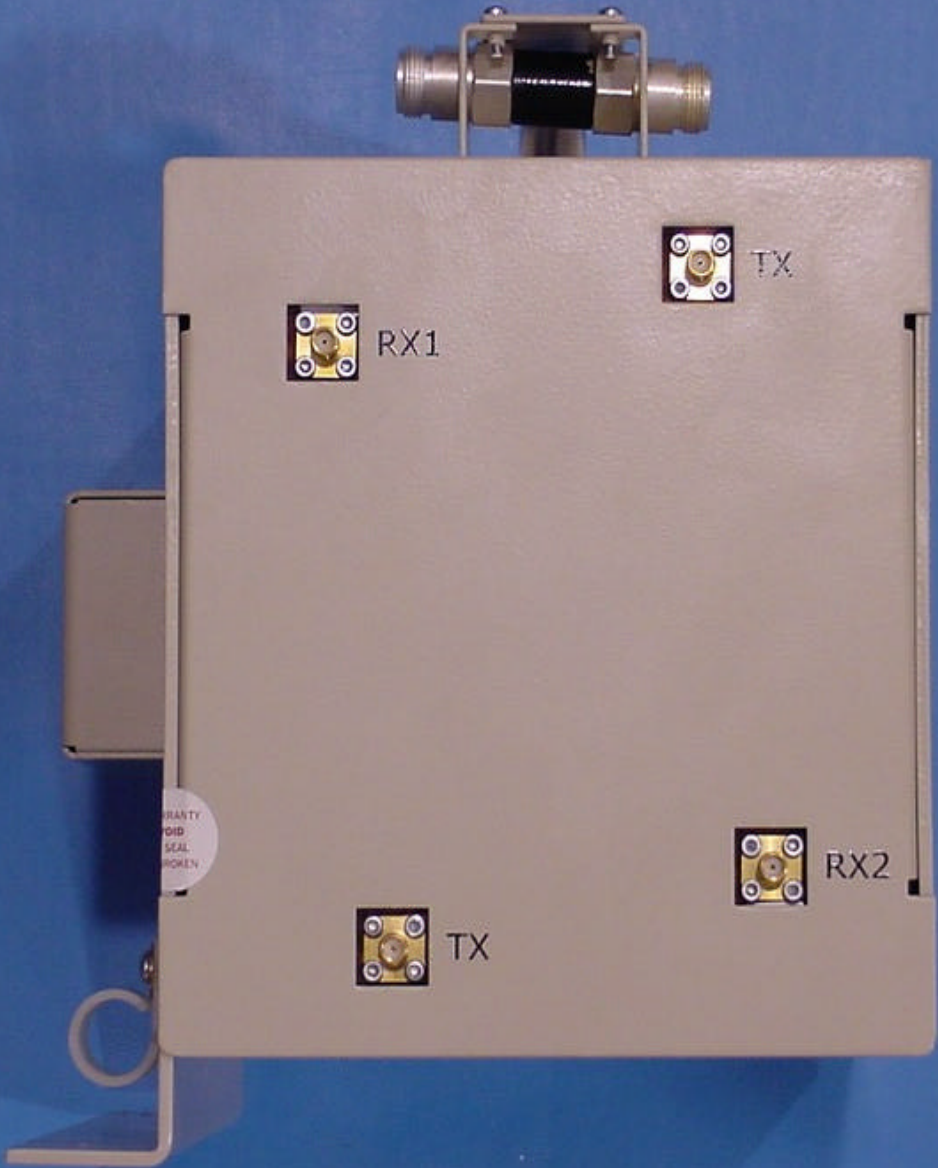
Digivance LRCS SMR Dual Transmit Duplexer Rear View
