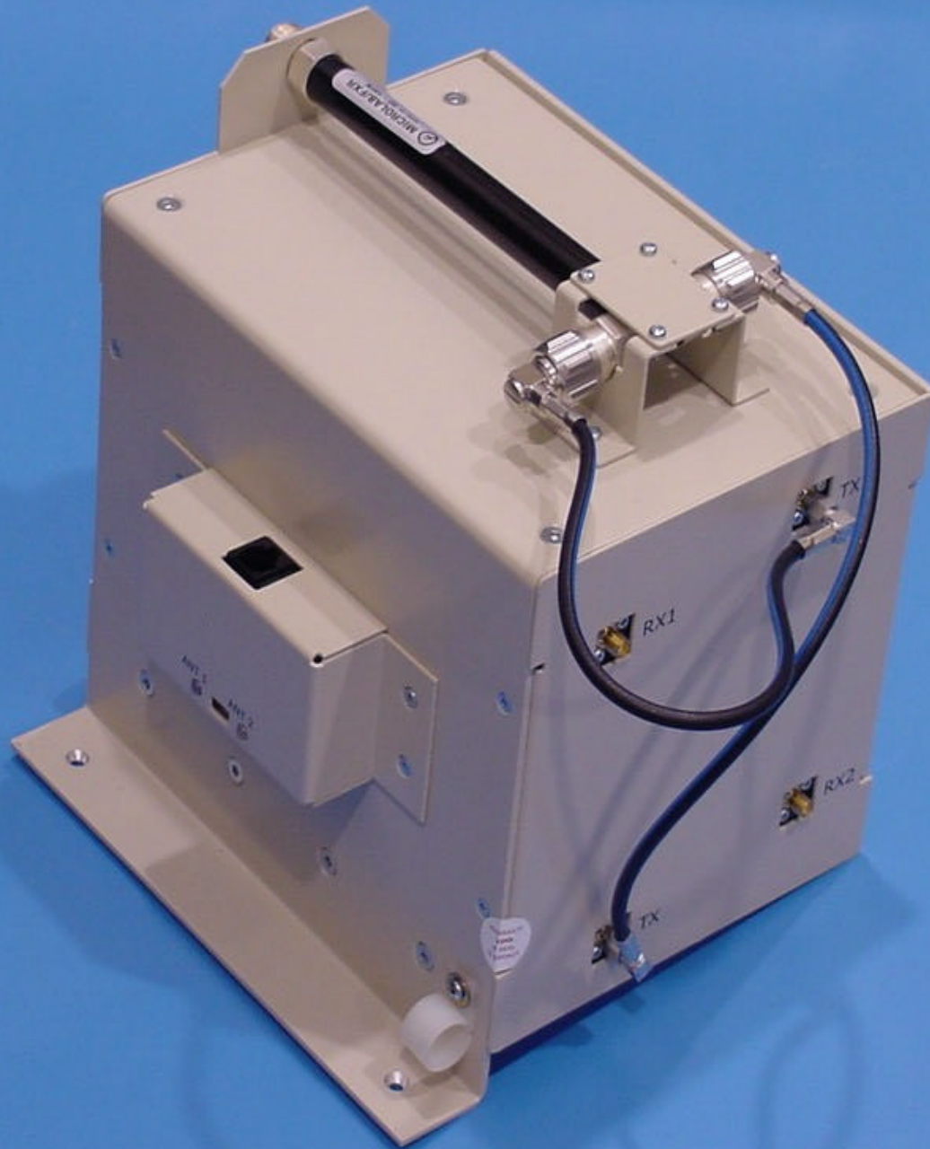
Digivance LRCS SMR Dual Transmit Duplexer Detail 2
