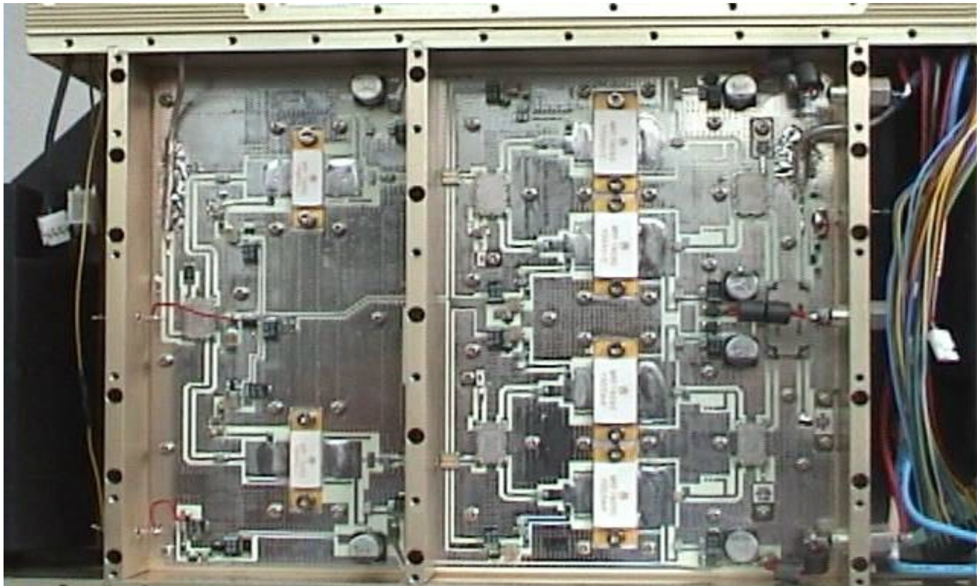
Digivance LRCS 1900 MHz Power Amplifier Main-Amp Board
