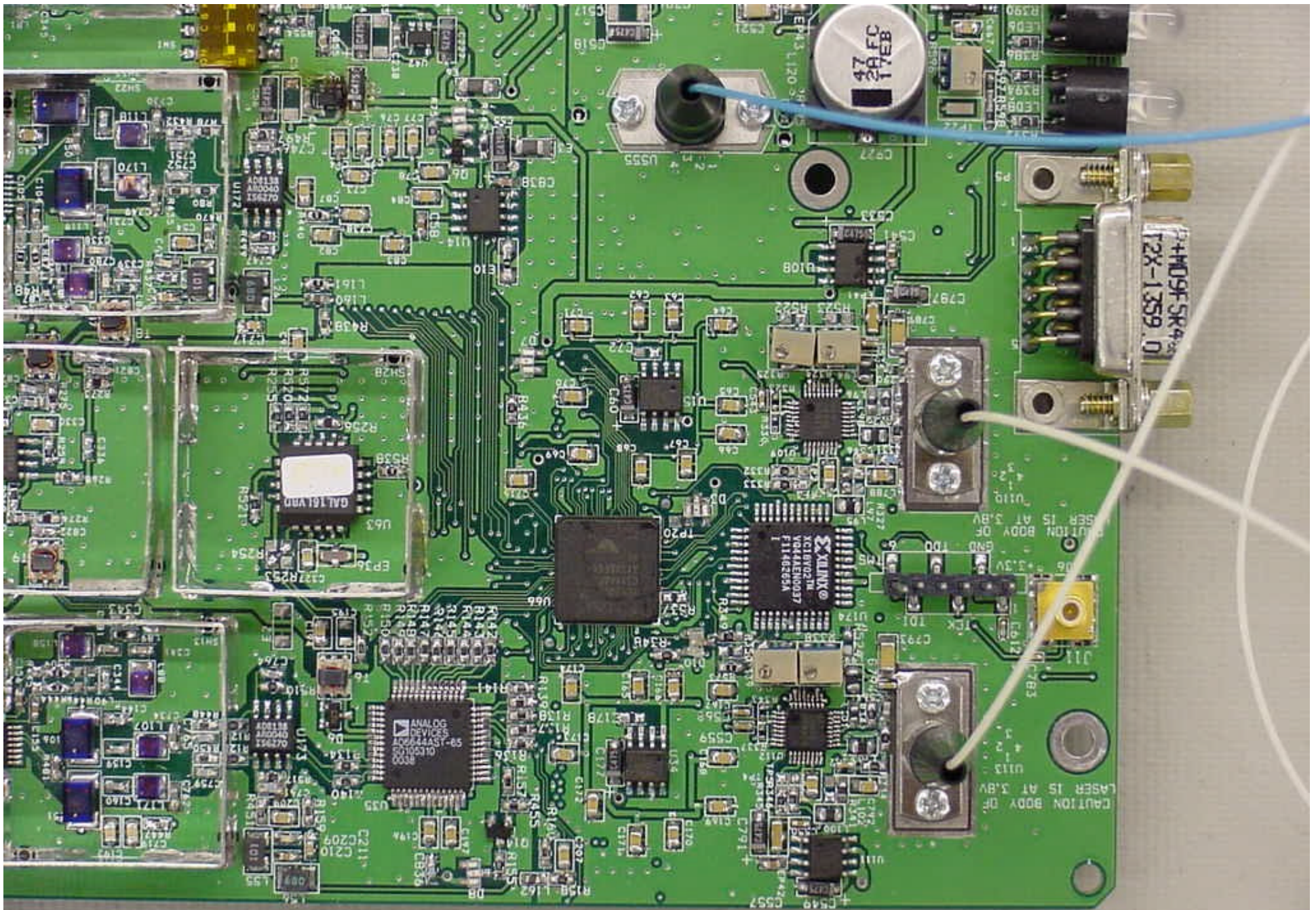
Digivance LRCS 800 MHz STM Control Board - T3
