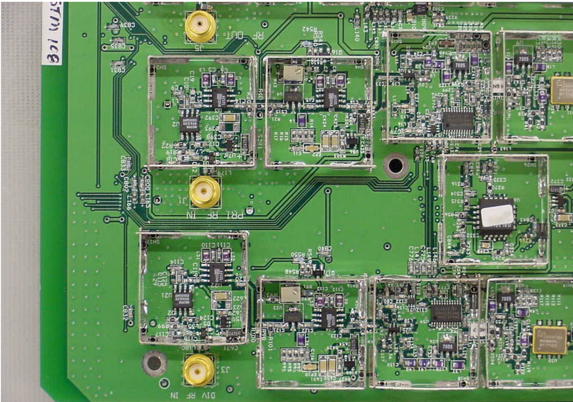
Digivance LRCS 800 MHz STM Control Board - T1
