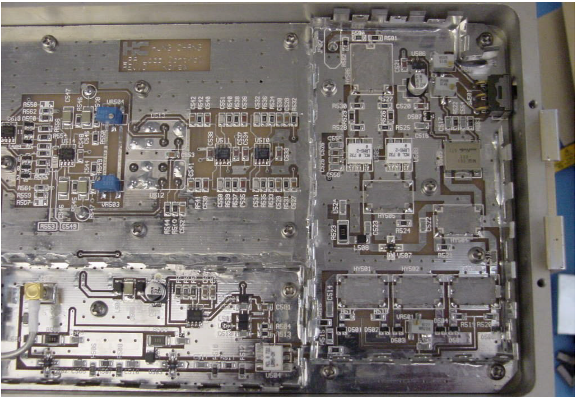
Digivance LRCS 800 MHz Power Amplifier - Loop Board - Top Right View
