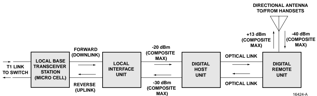
Figure 8. Local BTS Interface Block Diagram
