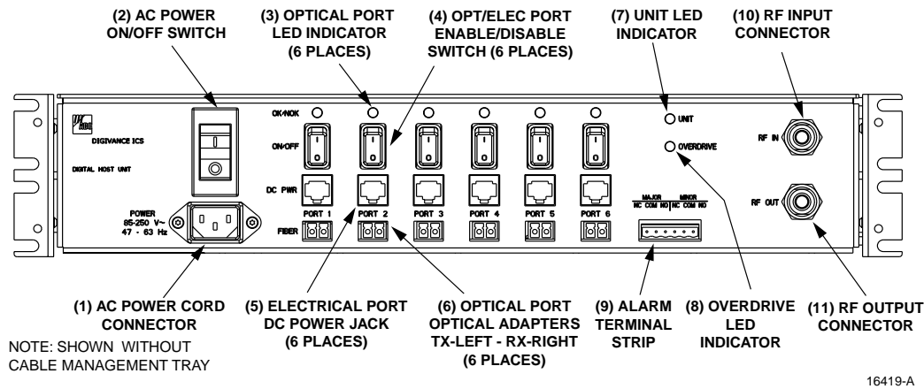
Figure 3. Digital Host Unit User Interface
