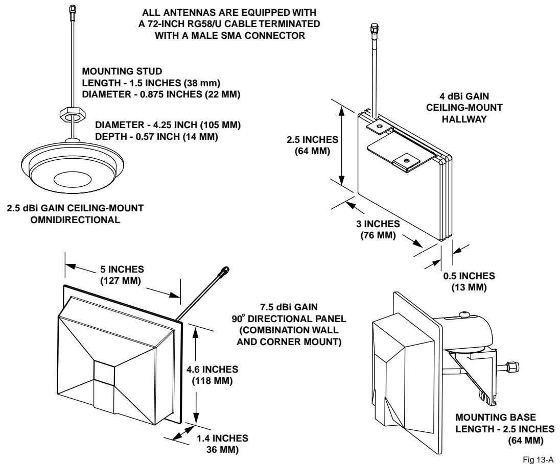
Figure 13. 1900 MHz DRU Antenna Options
