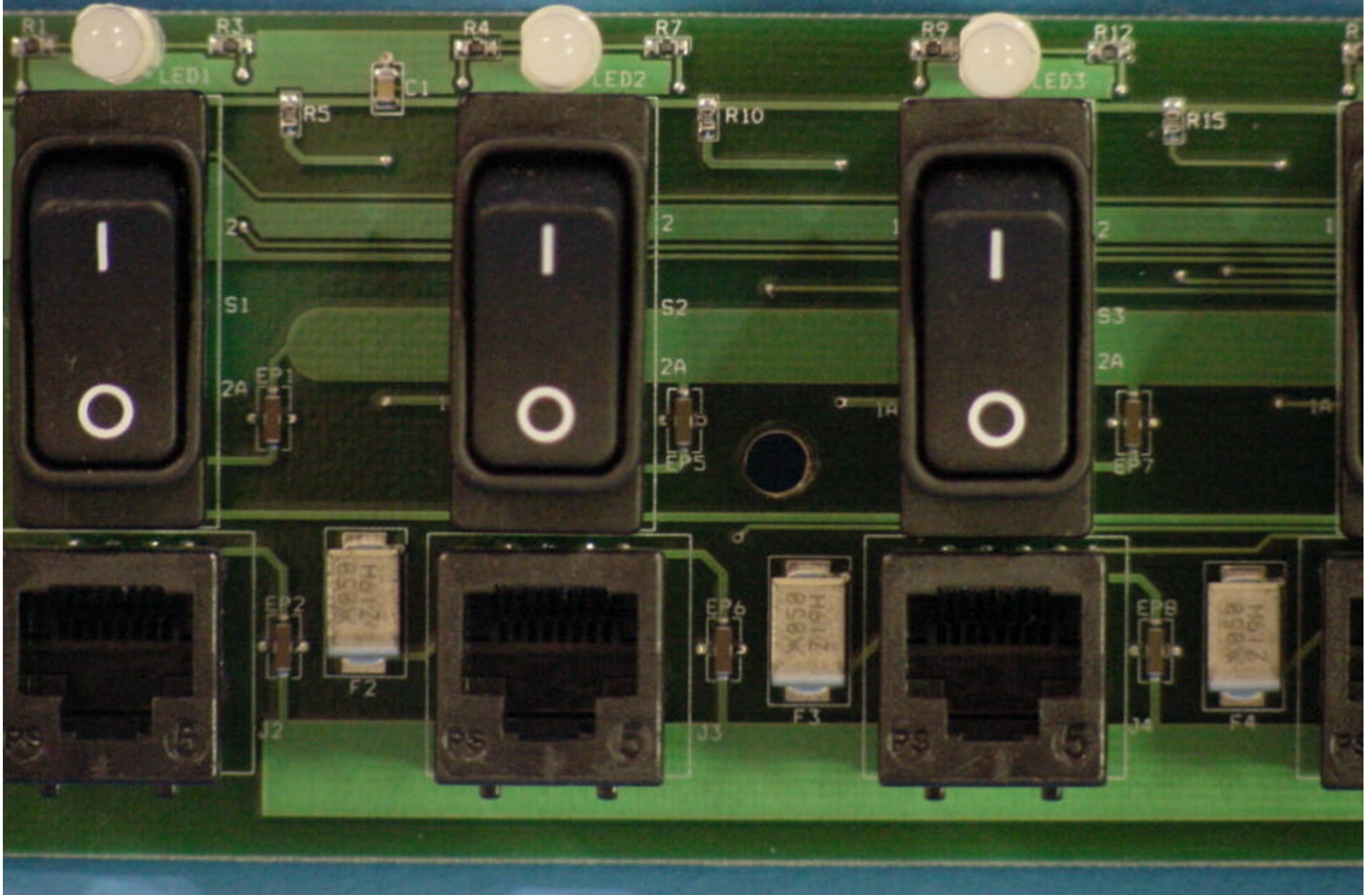
Digivance Digital Host Unit (DHU) Power Distribution Board Top Top Left Center
