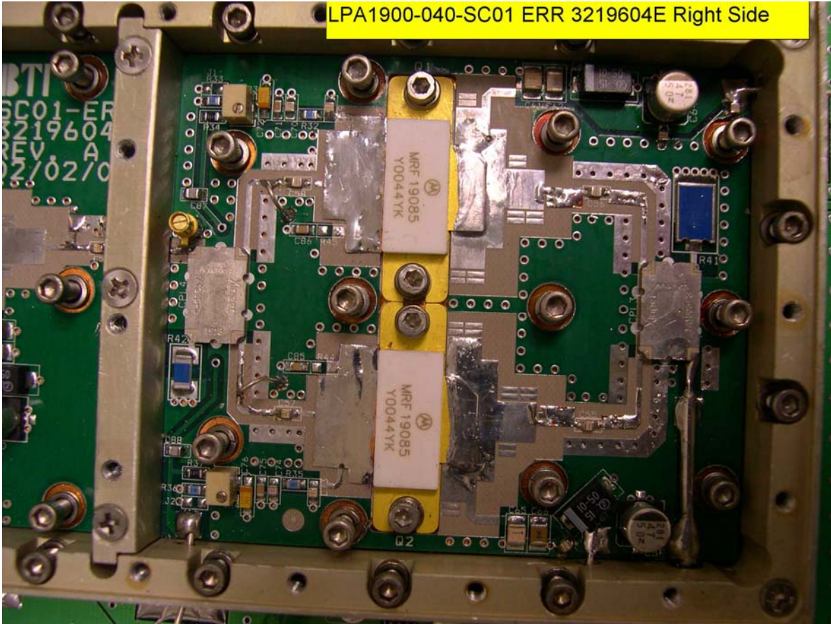
1900 MHz Linear Power Amplifier LPA1900-040-SC01-ERR 3219604E Right
