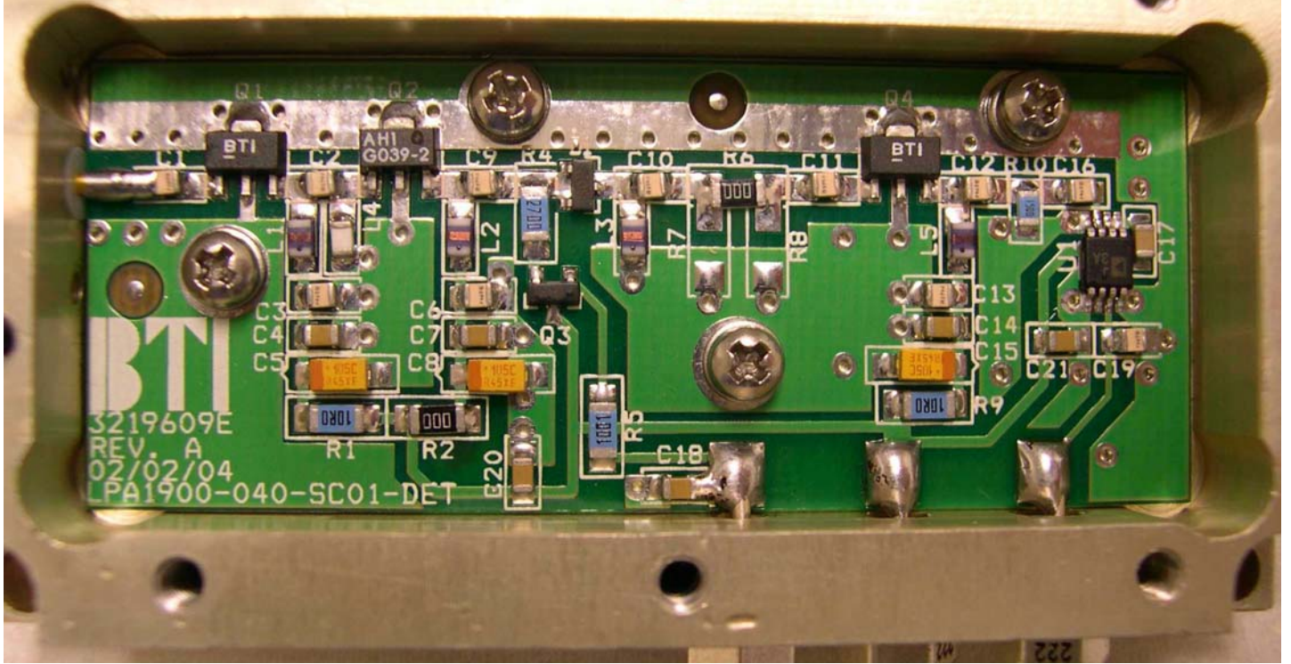
1900 MHz Linear Power Amplifier LPA1900-040-SC01-DET 3219609E
