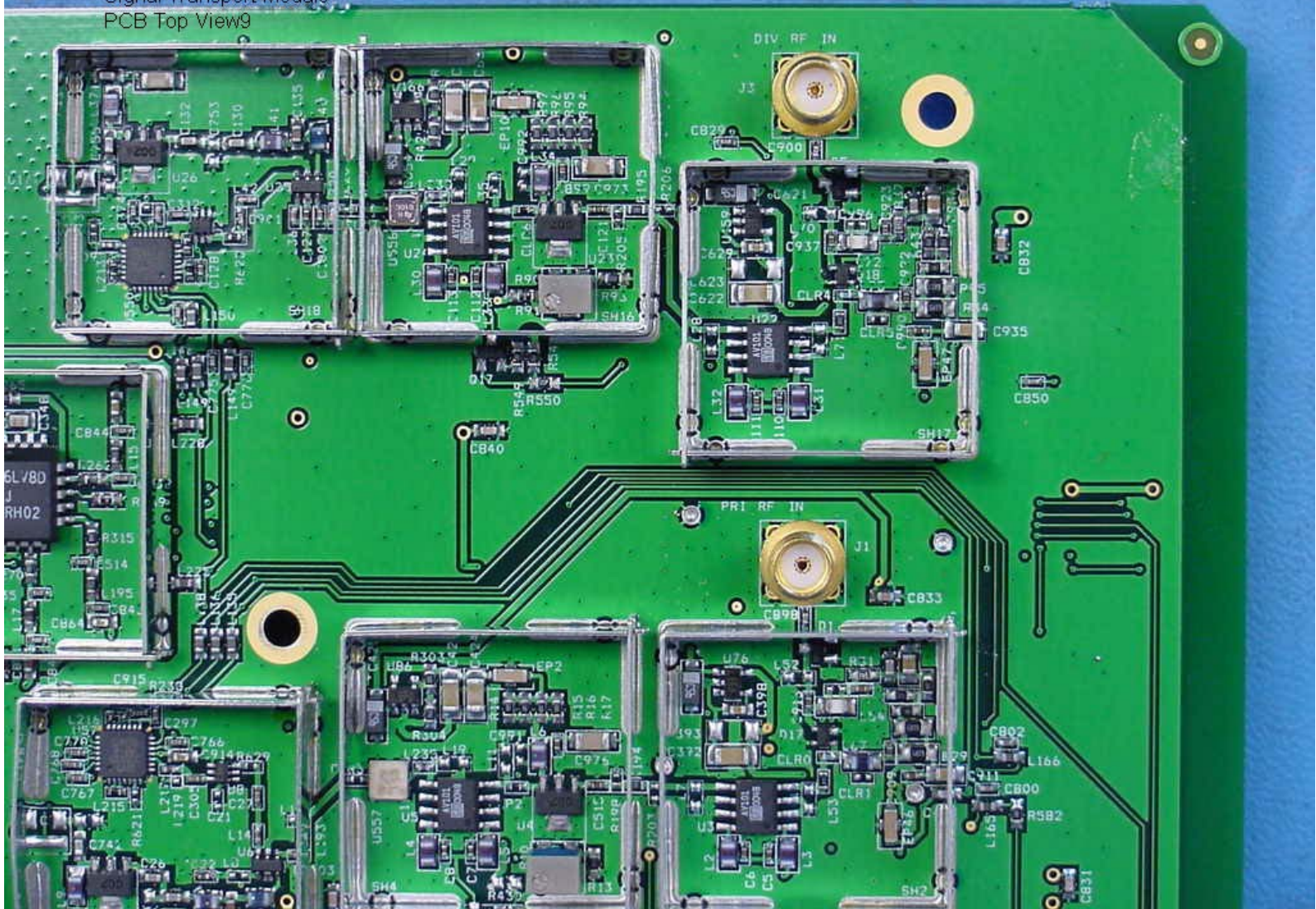
Digivance LRCS 1900 MHz STM Board Top View 9
