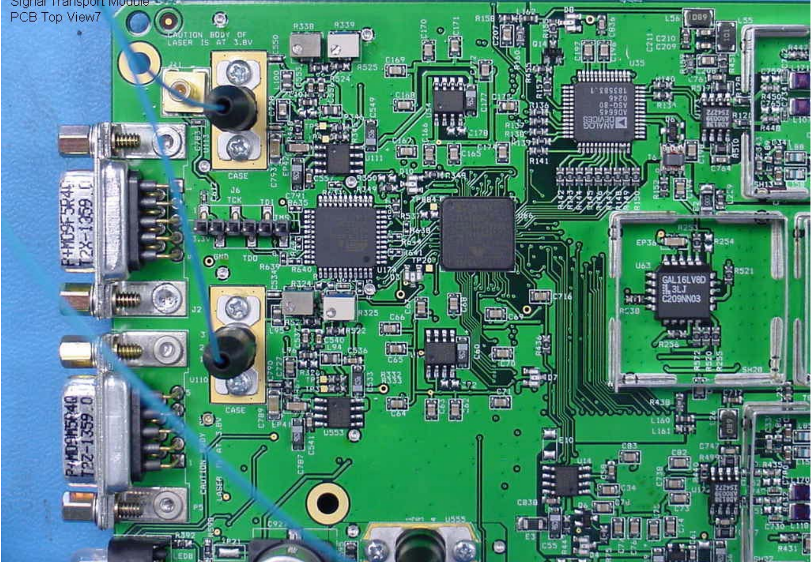
Digivance LRCS 1900 MHz STM Board Top View 7
