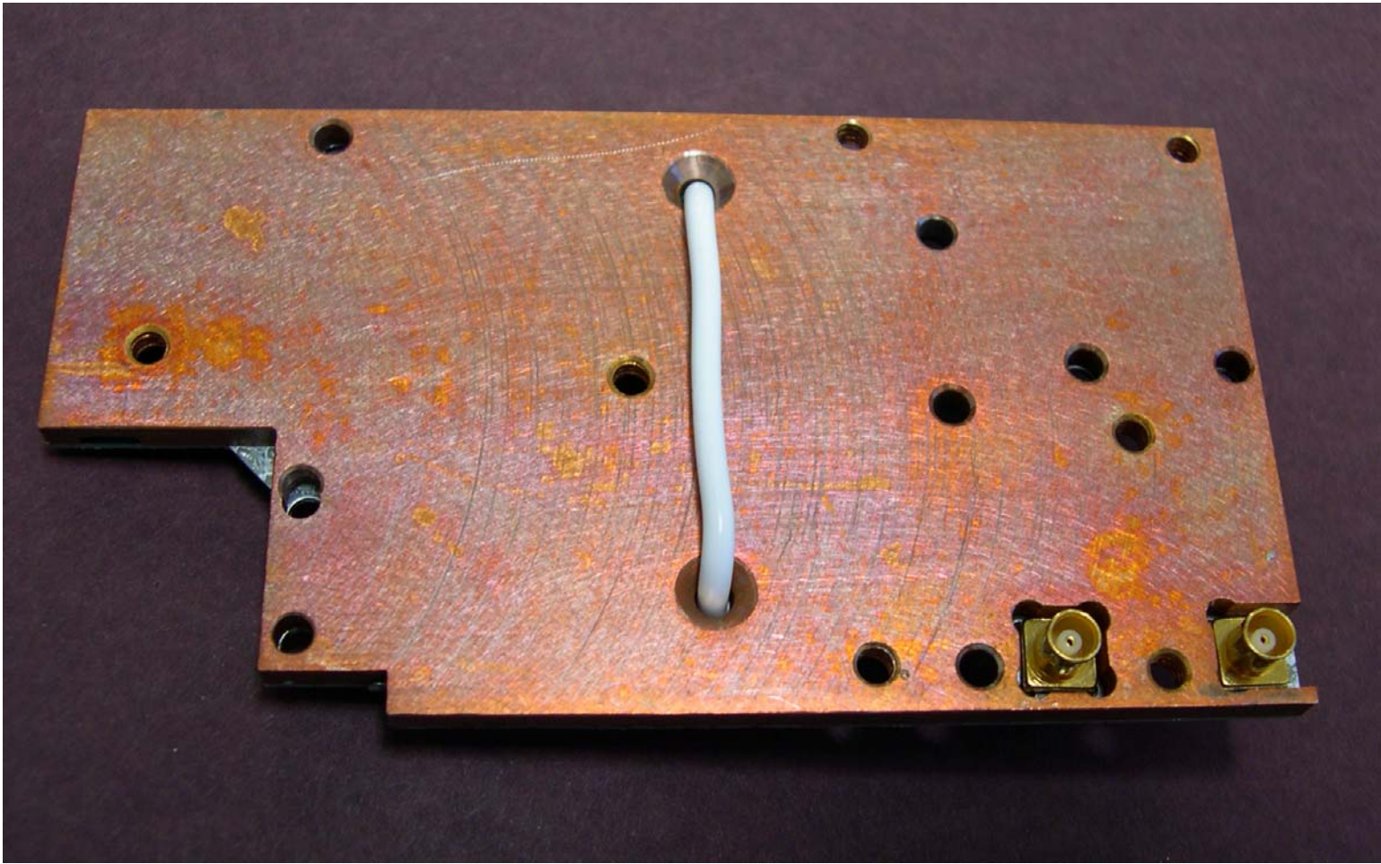
Digivance Street Coverage Solution (SCS) Power Amplifier 4244601E Rev A Board Back
