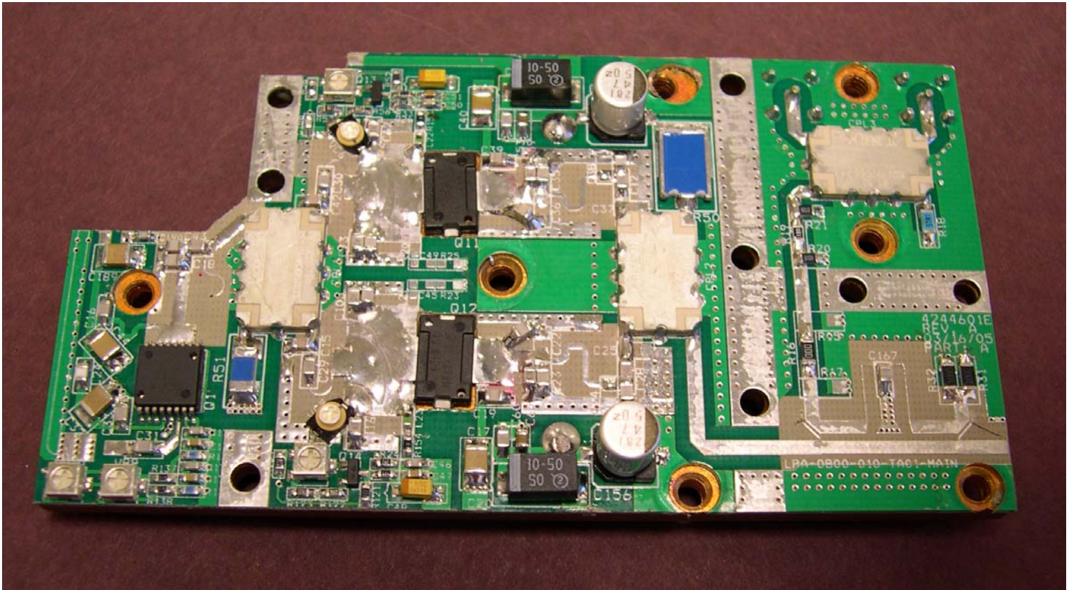
Digivance Street Coverage Solution (SCS) Power Amplifier 4244601E Rev A Board Front
