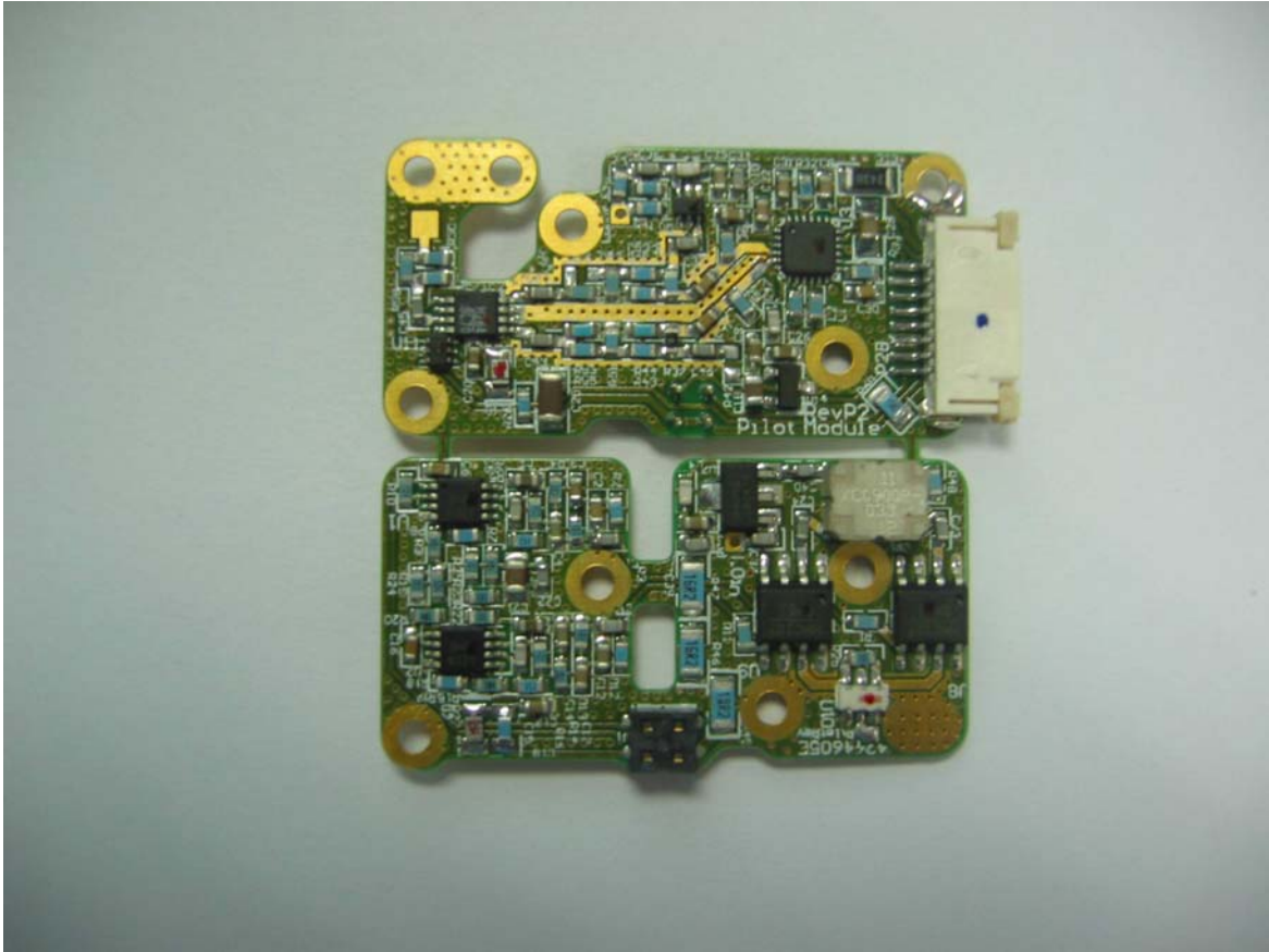
Linear Power Amplifier 10 Watt Pilot Tone, Part A - Top
