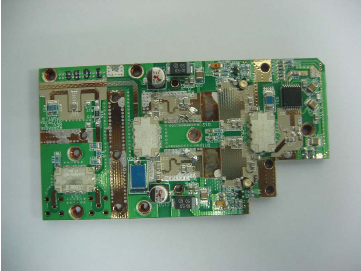
Linear Power Amplifier 10 Watt Main Board, Part A – Top
