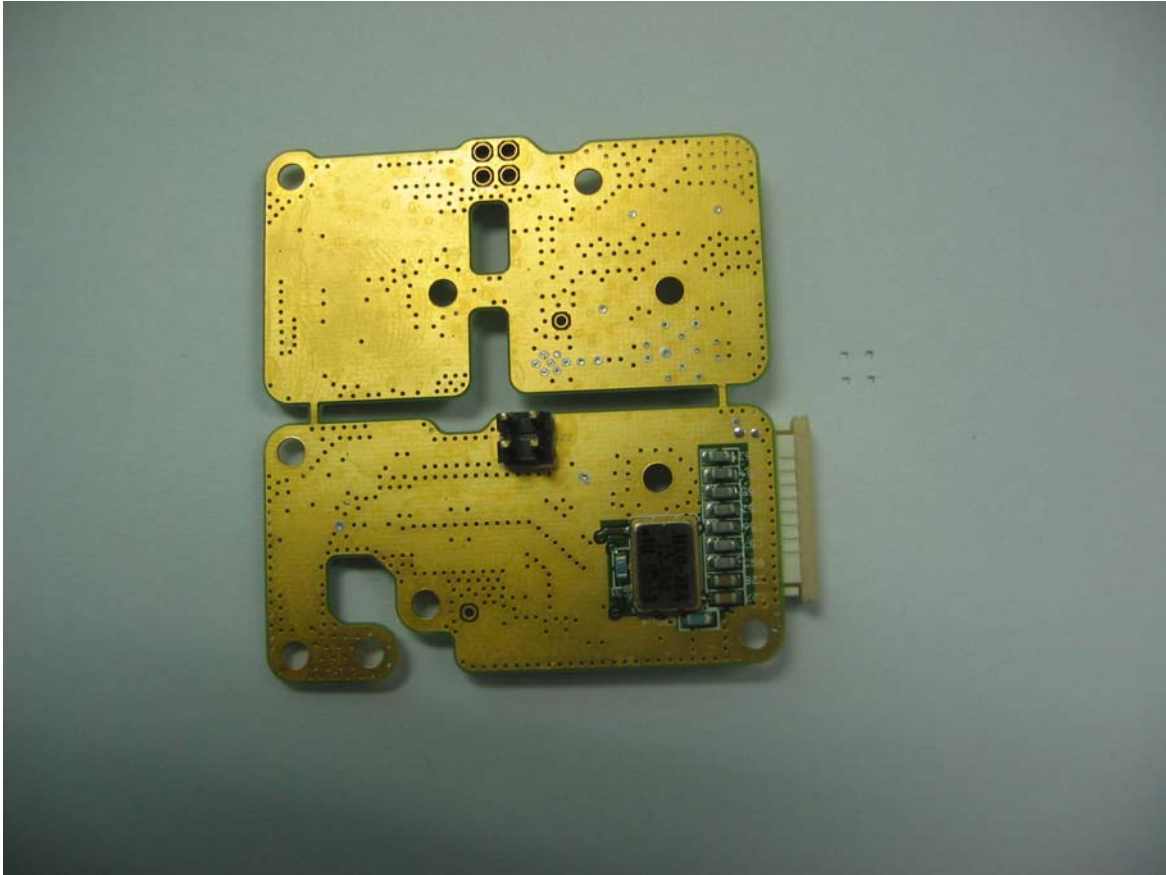
Linear Power Amplifier 10 Watt Pilot Tone, Part A - Bottom
