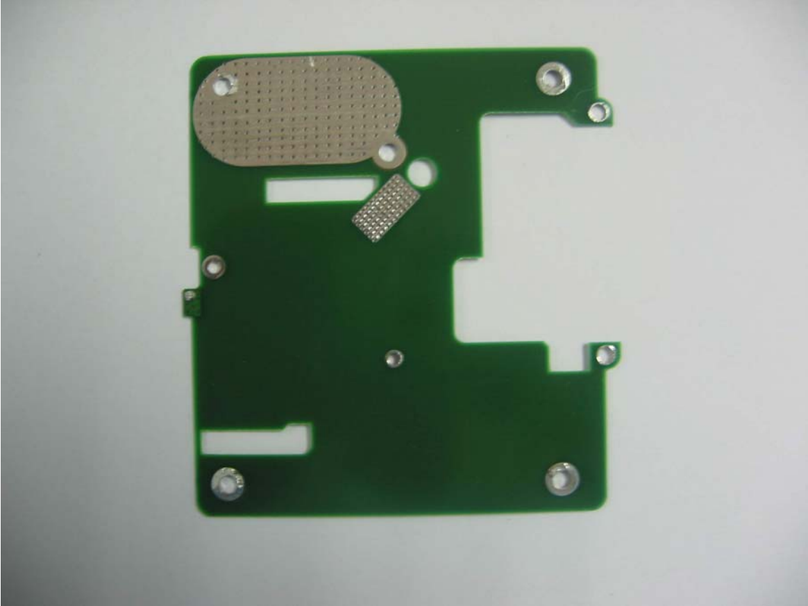
Linear Power Amplifier 10 Watt Mother Board, Part B - Bottom
