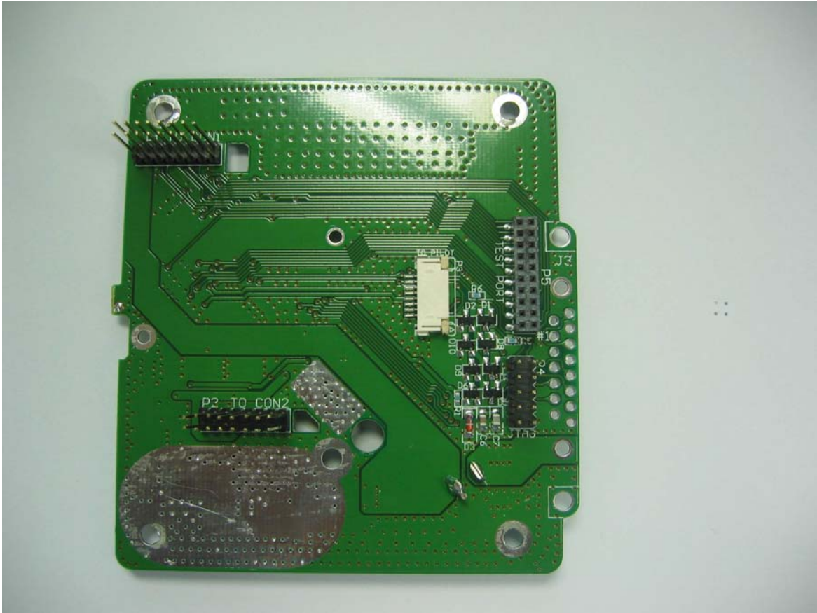
Linear Power Amplifier 10 Watt Mother Board, Part A - Bottom
