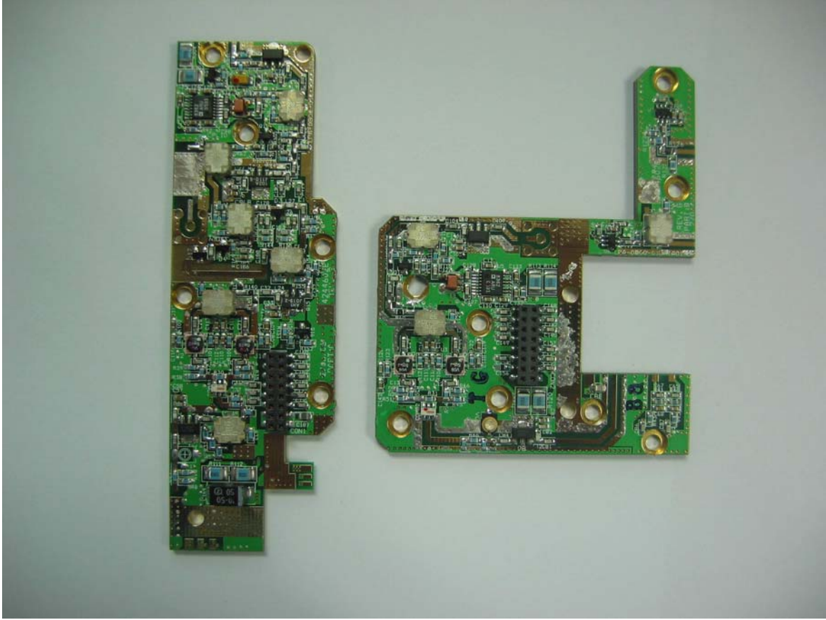
Linear Power Amplifier 10 Watt Driver Board, Part A - Top
