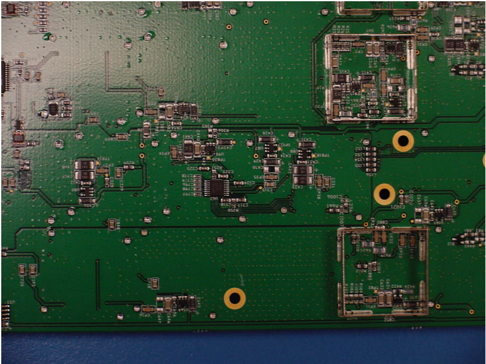
Digivance 1900 MHz Remote Board Bottom View 2
