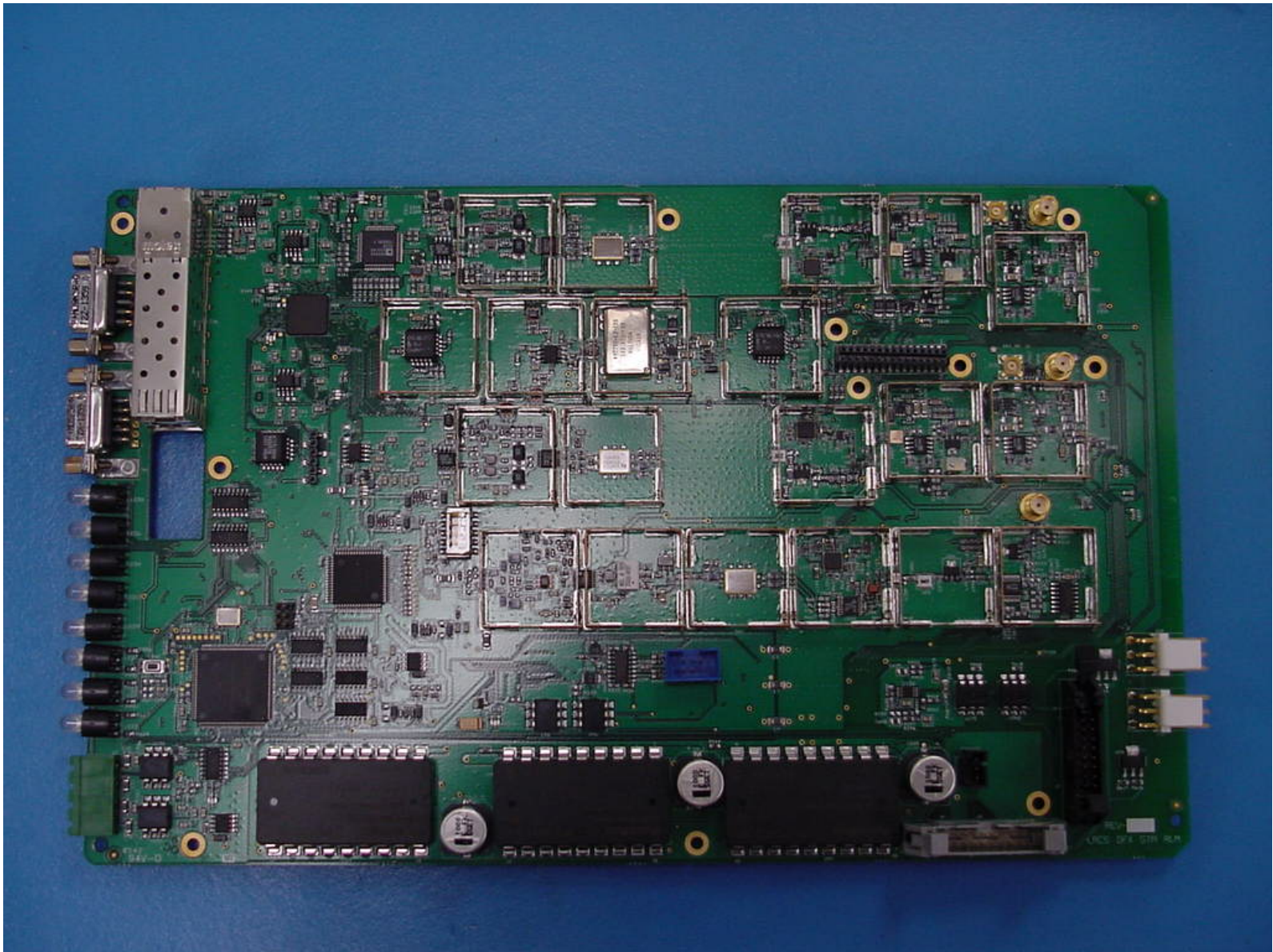
Digivance 1900 MHz Remote Board Top View
