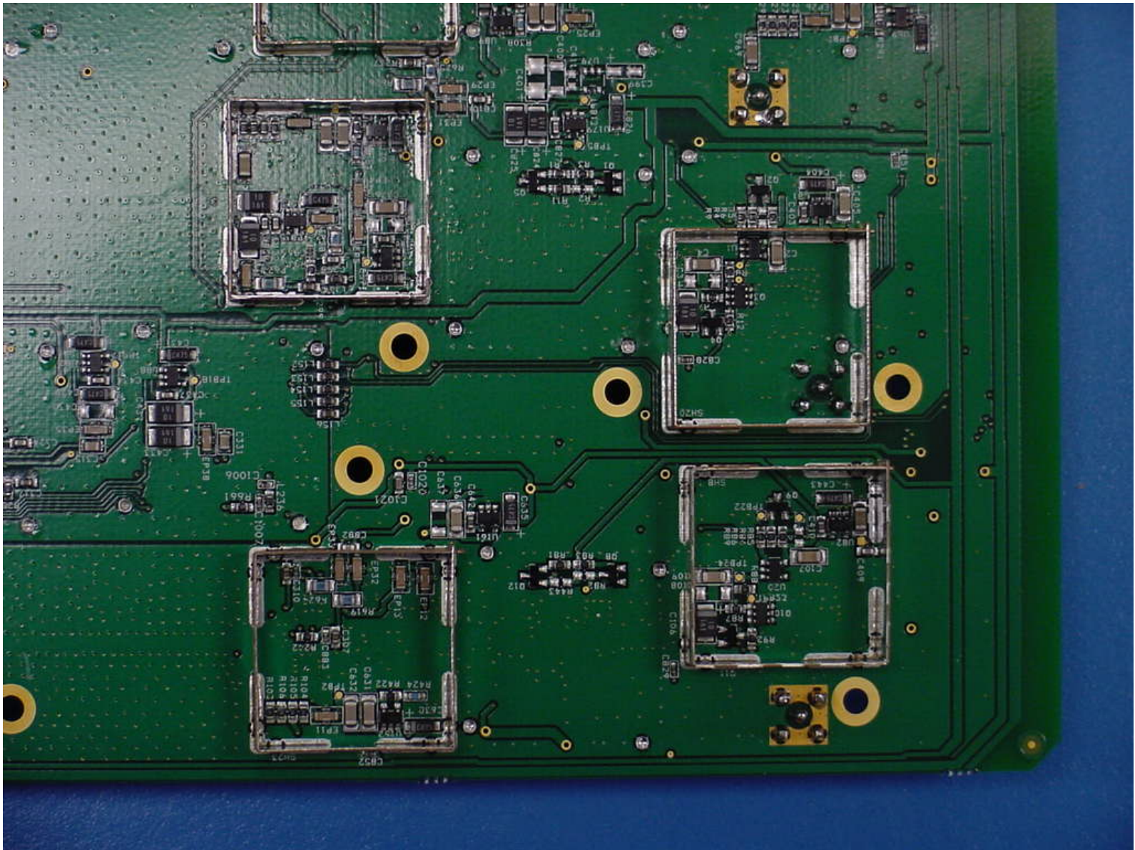
Digivance 1900 MHz Remote Board Bottom View 3
