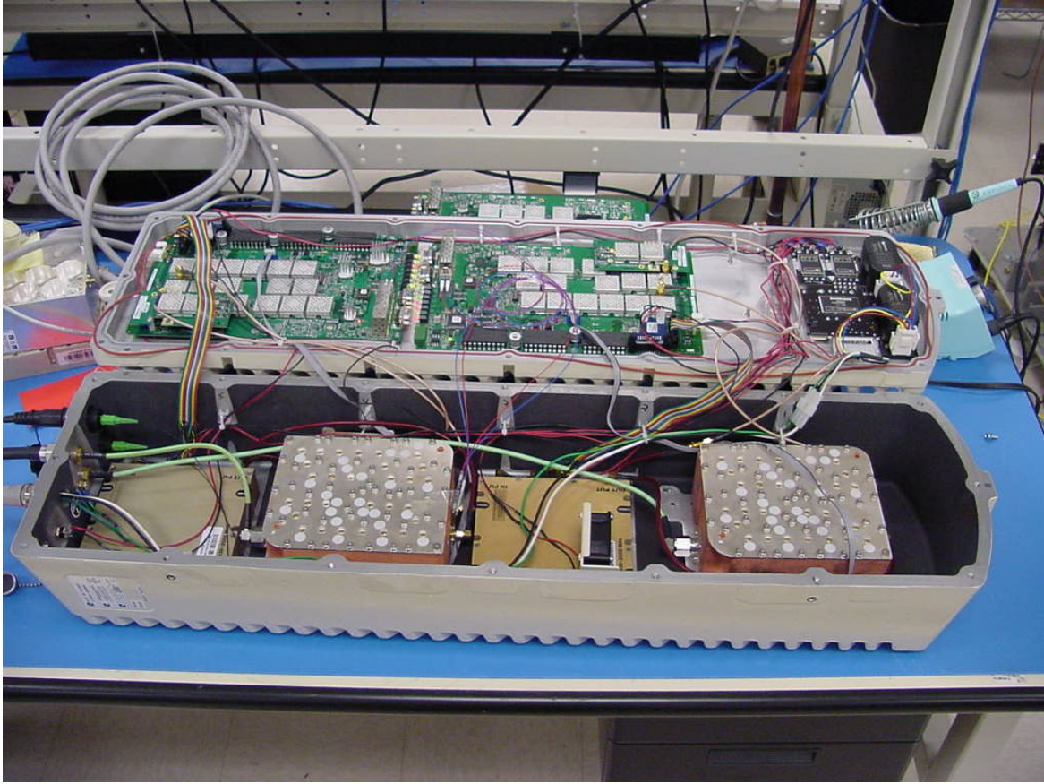
Digivance SCS – PCS/PCS Remote Unit Open View
