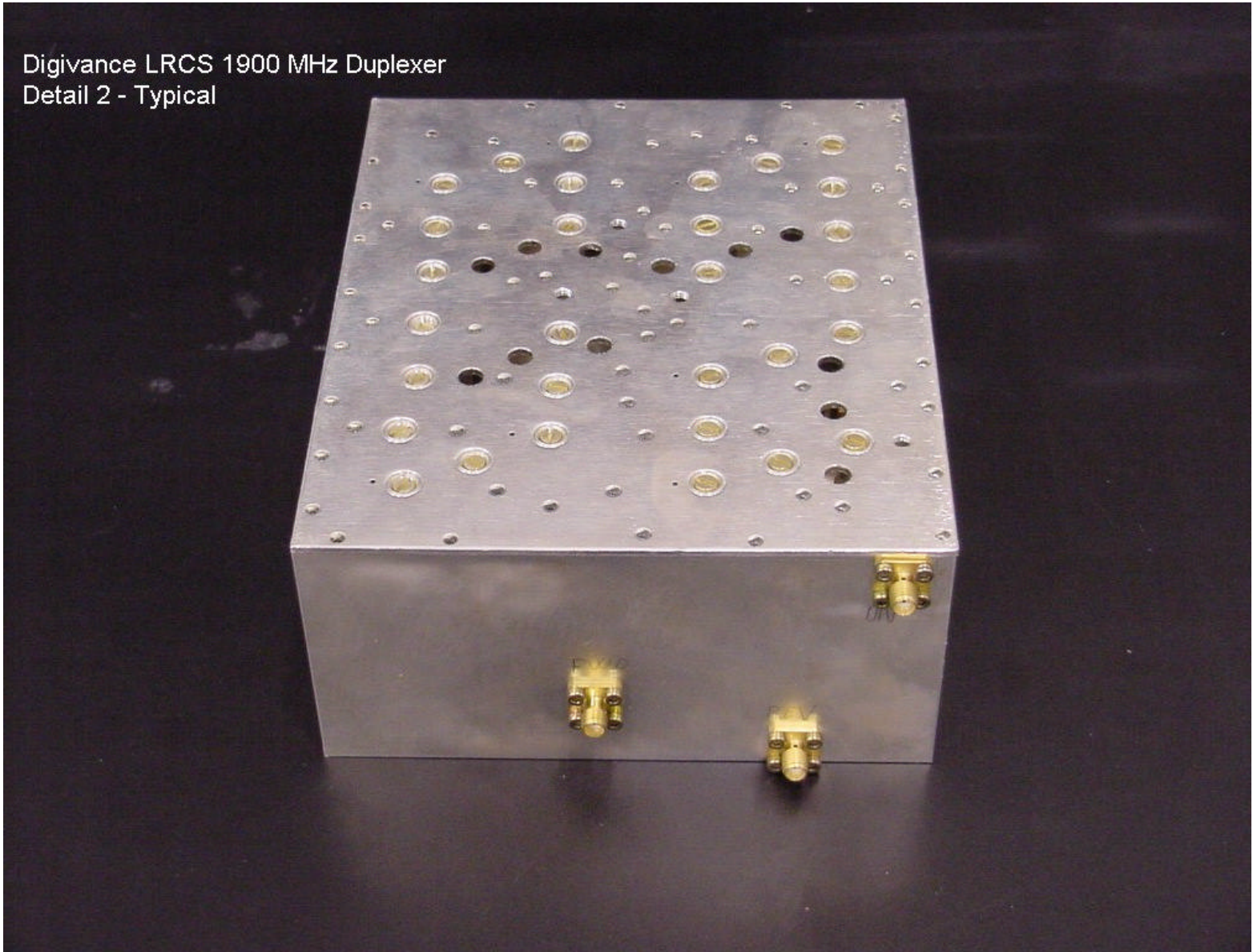
Digivance LRCS 1900 MHz Duplexer Rear View
