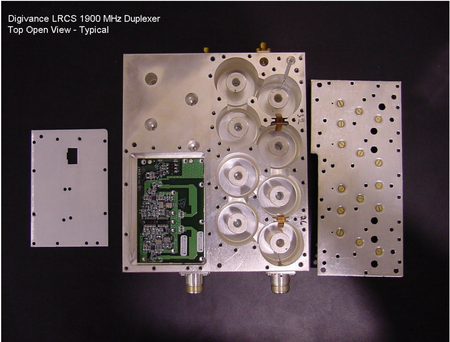
Digivance LRCS 1900 MHz Duplexer Top Open View
