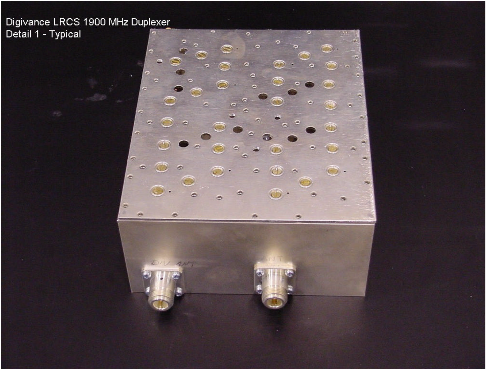
Digivance LRCS 1900 MHz Duplexer Front View
