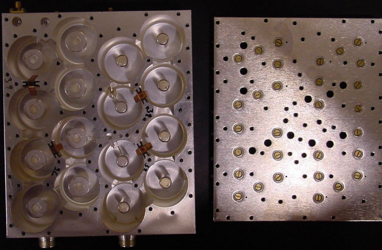
Digivance LRCS 1900 MHz Duplexer Bottom Open View - Typical
