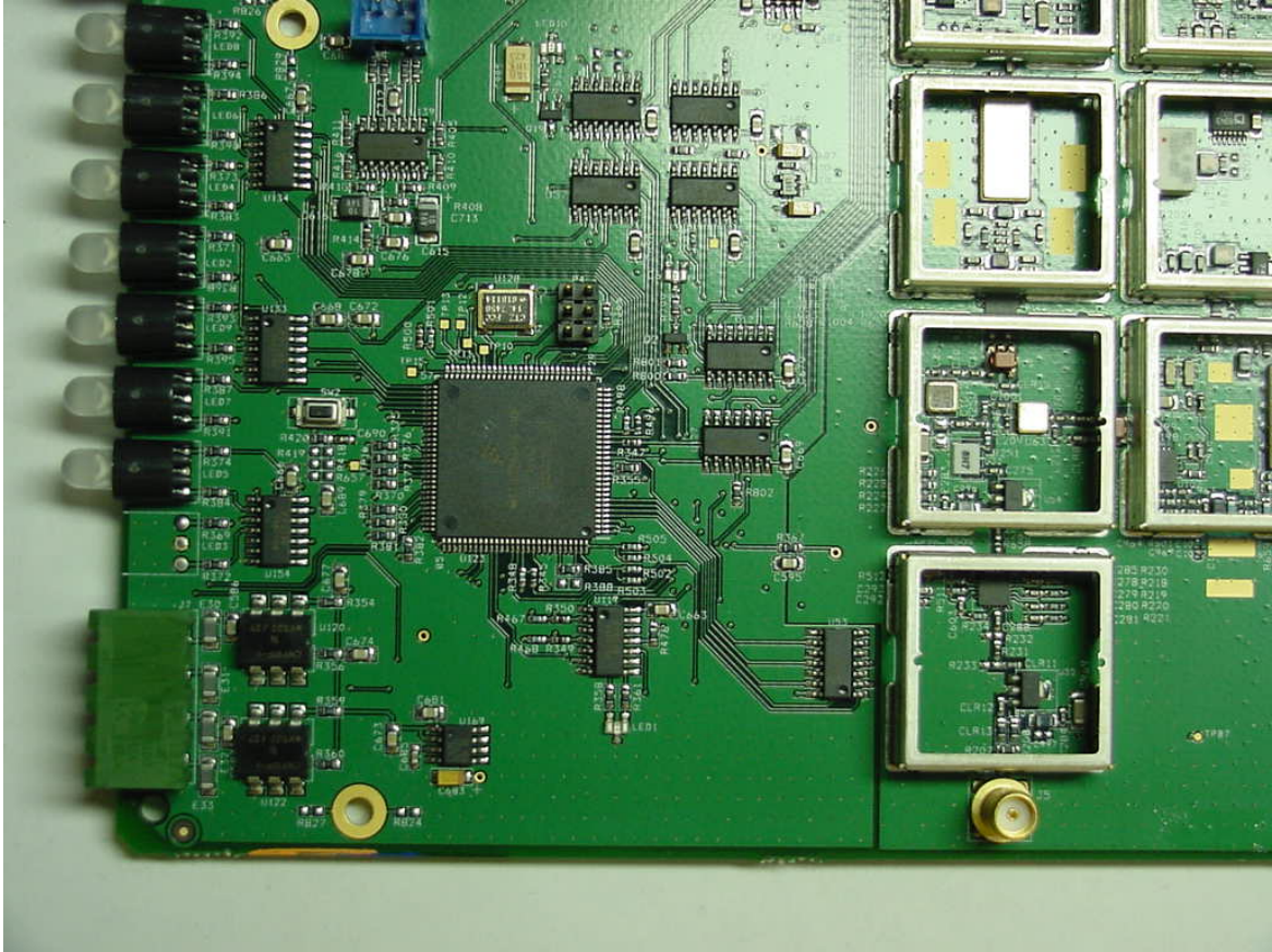
SMR Dual Band Remote Board Top View 1
