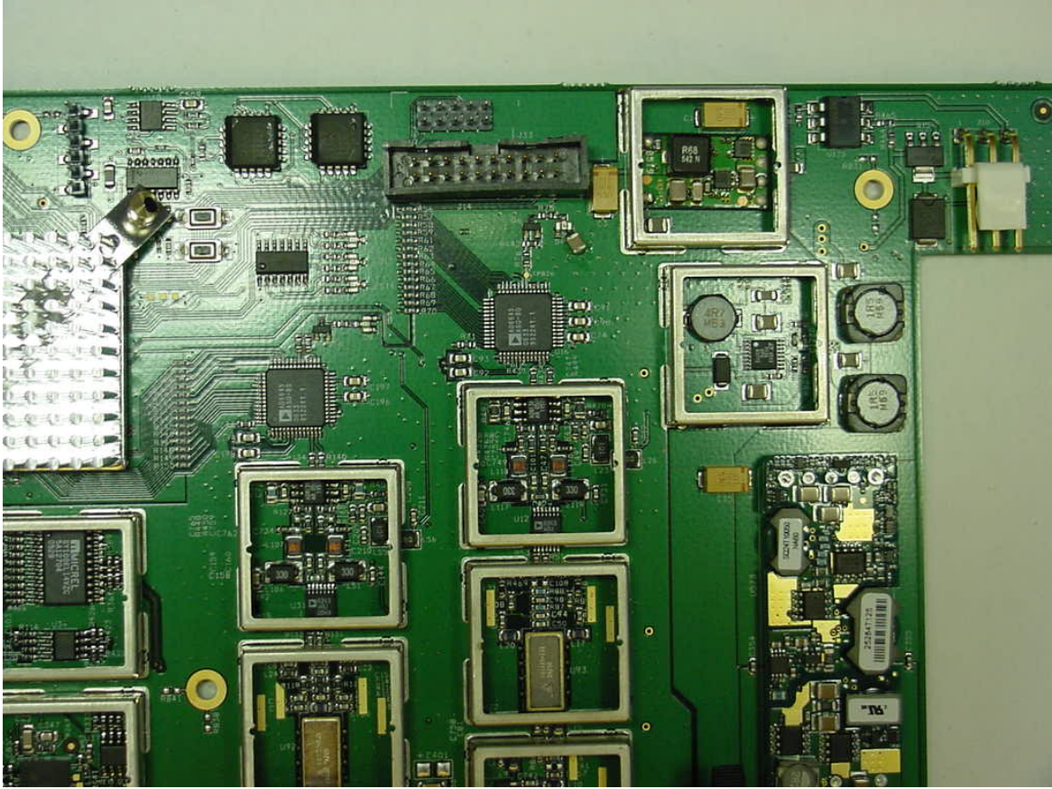
SMR Dual Band Remote Board Top View 4
