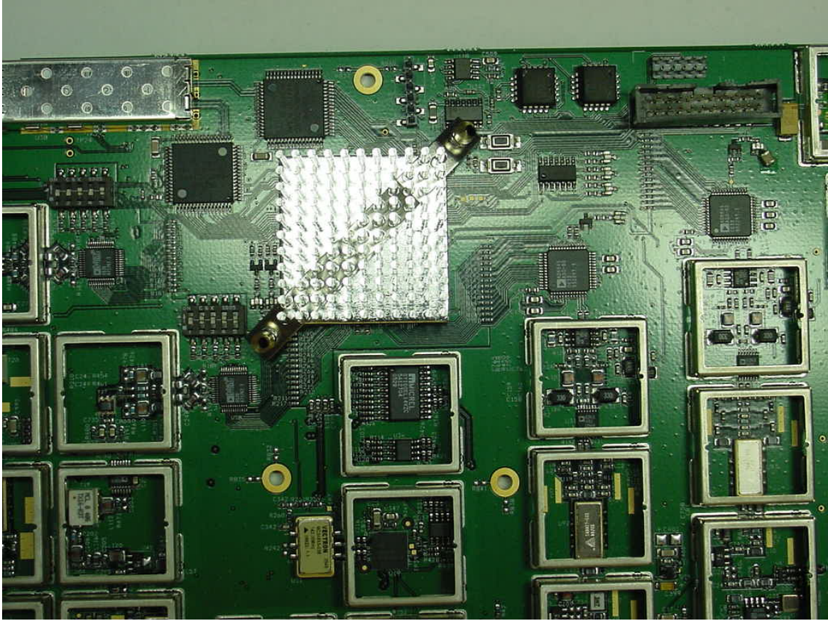
SMR Dual Band Remote Board Top View 5
