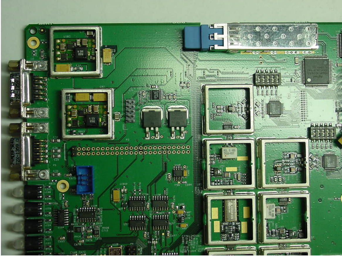
SMR Dual Band Remote Board Top View 6
