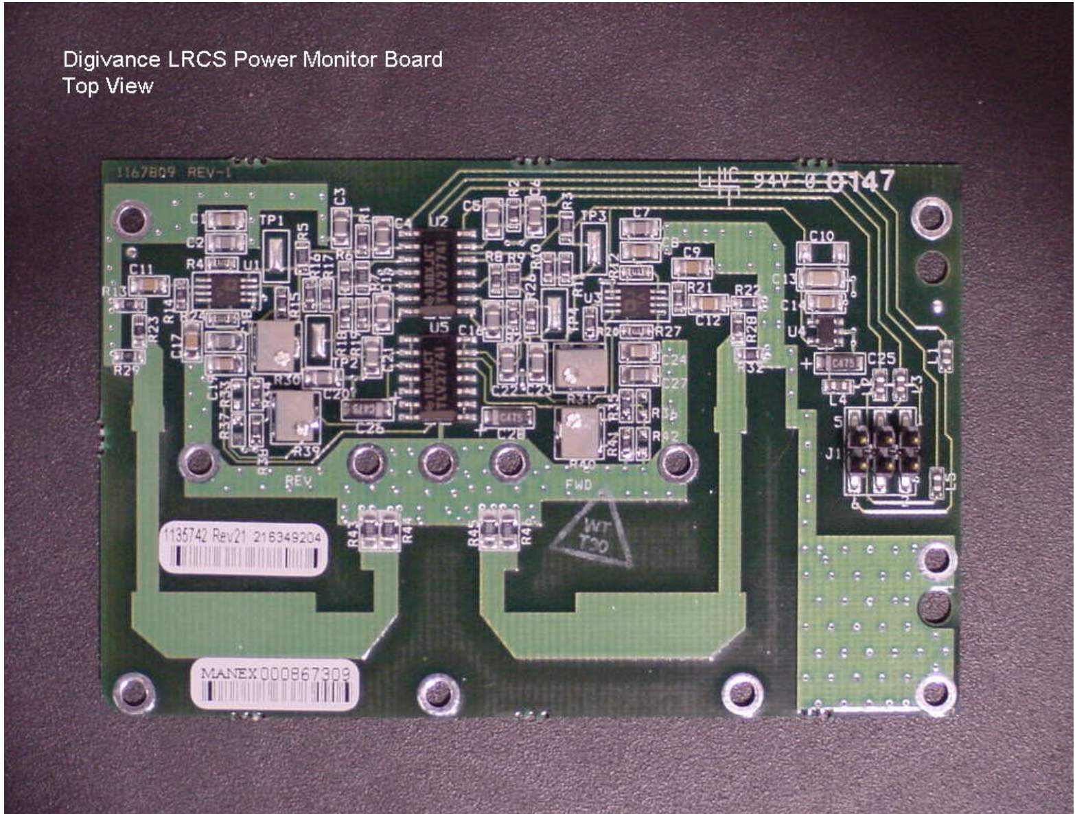
Digivance LRCS Power Monitor Board Top View
