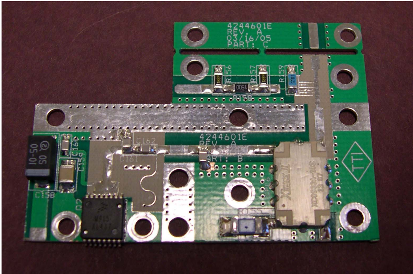
Bravo Tech SMR 800/900 Dual Band Linear Power Amplifier - 10 Watt Board 4244601E Rev A Part B_C
