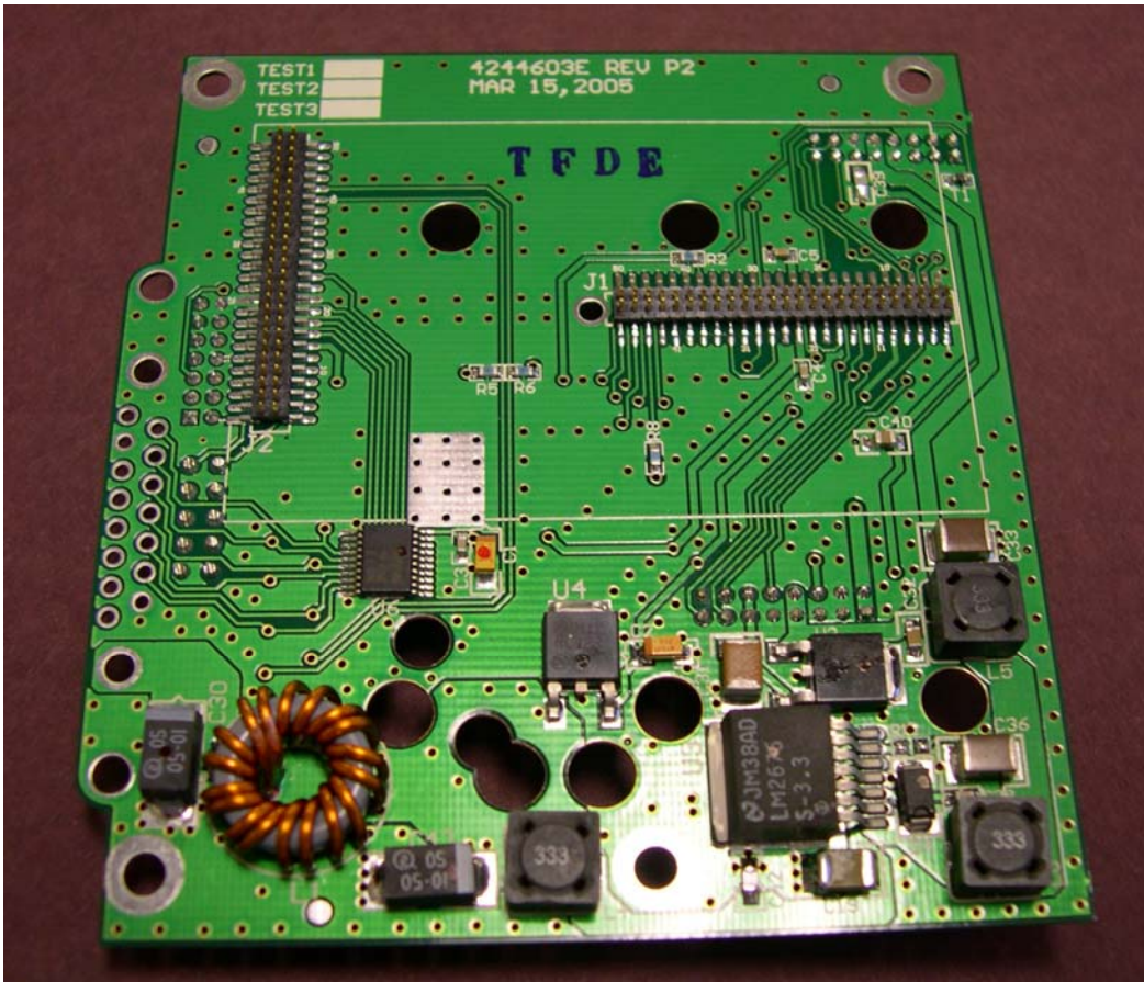
Bravo Tech SMR 800/900 Dual Band Linear Power Amplifier - 10 Watt Board 4244603E-Rev P2
