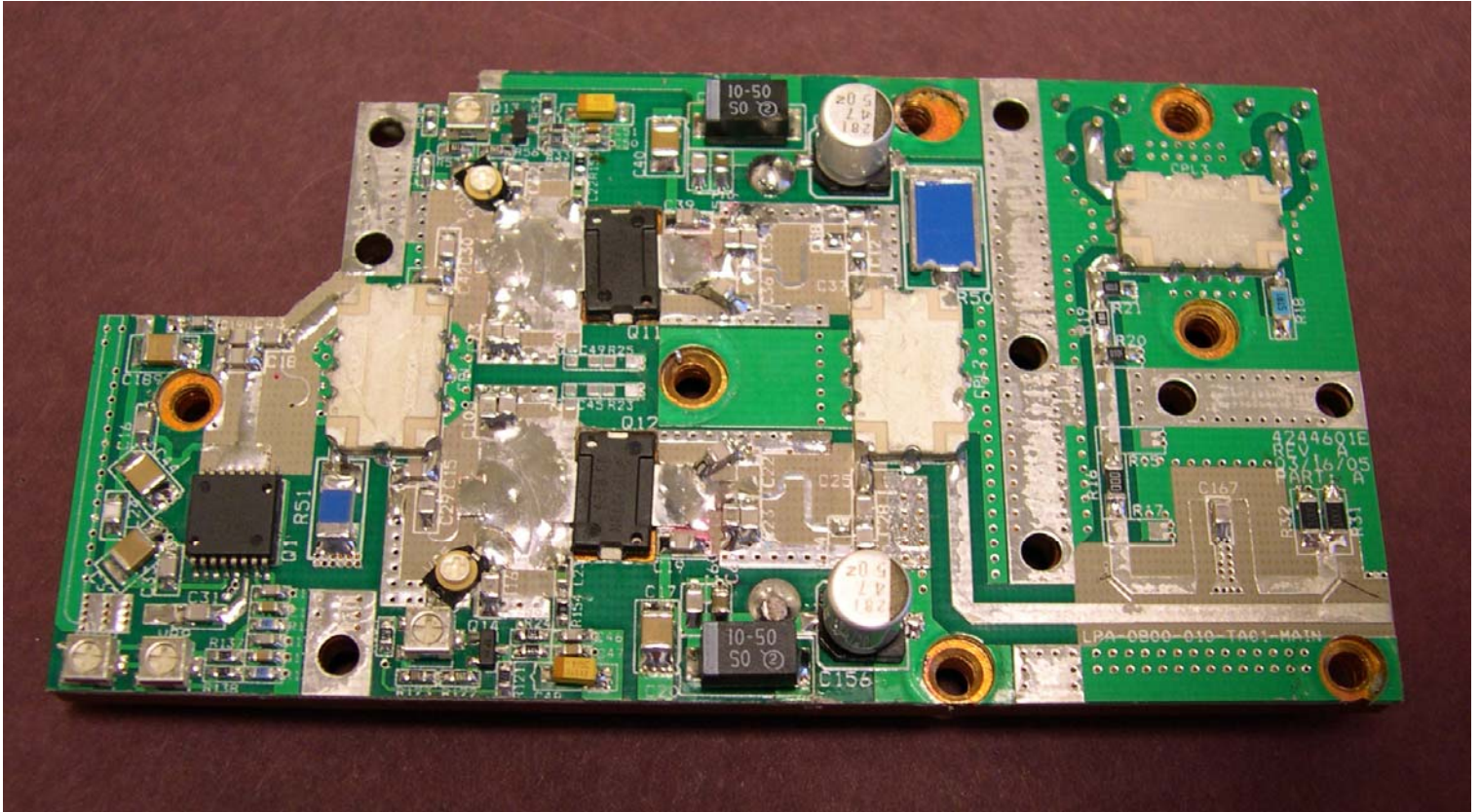
Bravo Tech SMR 800/900 Dual Band Linear Power Amplifier - 10 Watt Board 4244601E - Rev A
