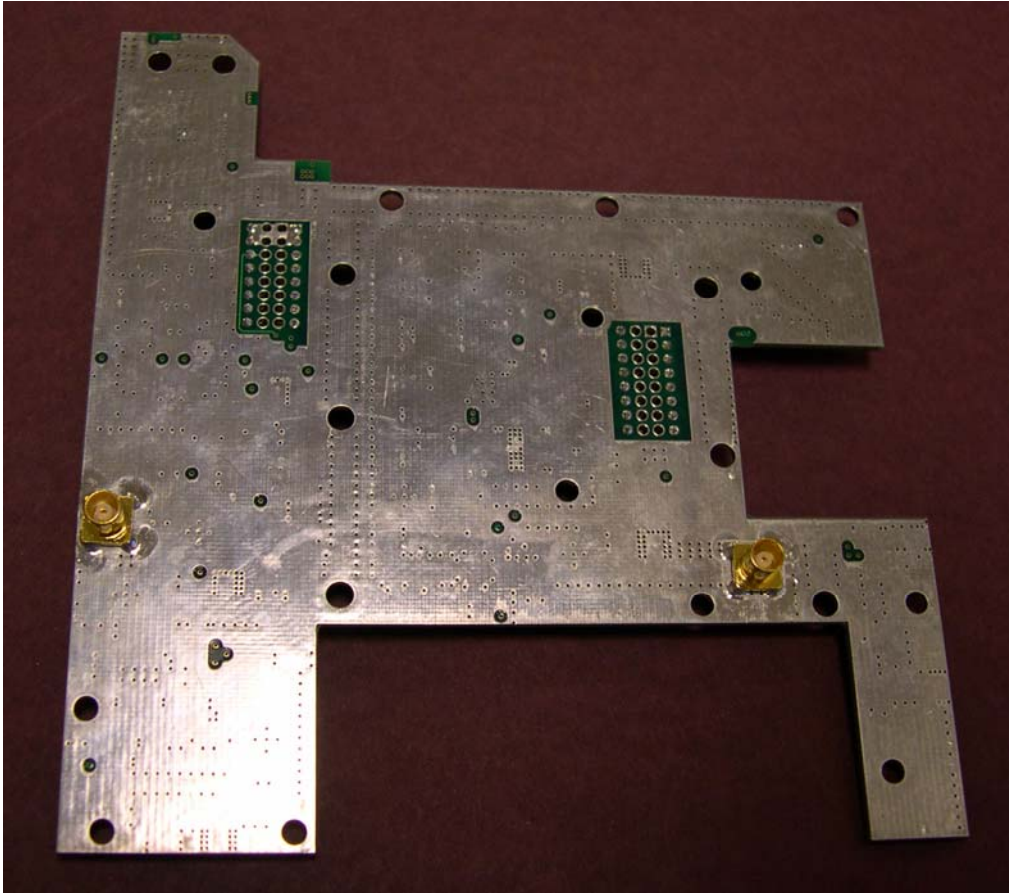
Bravo Tech SMR 800/900 Dual Band Linear Power Amplifier - 10 Watt Back of Board 4244602E Rev A
