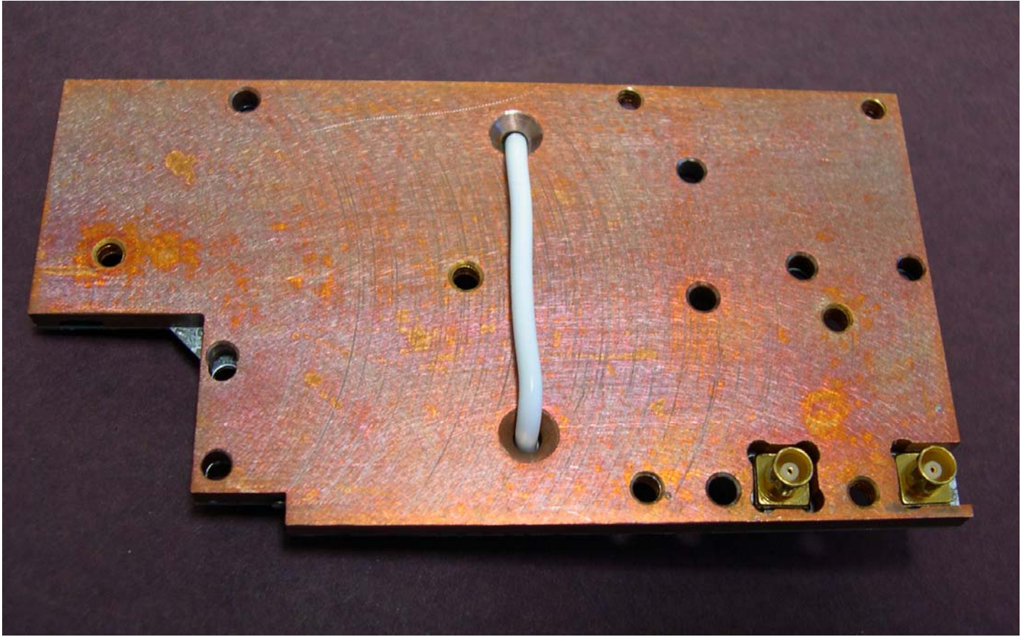
Bravo Tech SMR 800/900 Dual Band Linear Power Amplifier - 10 Watt Back of Board 4244601E - Rev A
