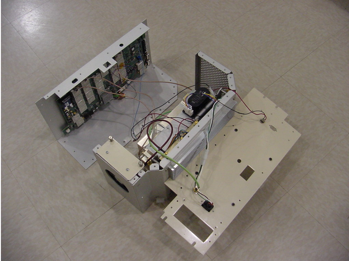
Digivance SCX - SMR Remote Unit Open View – Bottom Right
