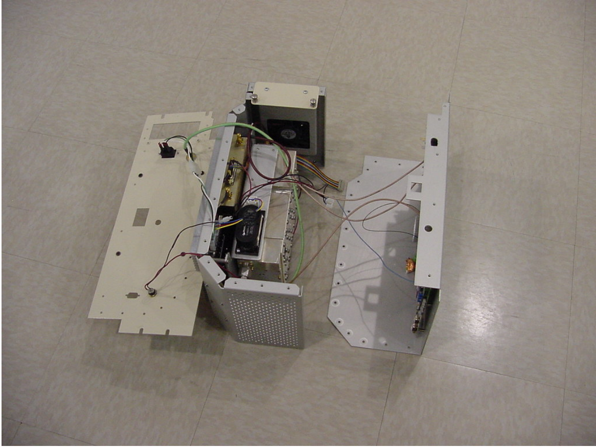
Digivance SCX - SMR Remote Unit Open View – Top
