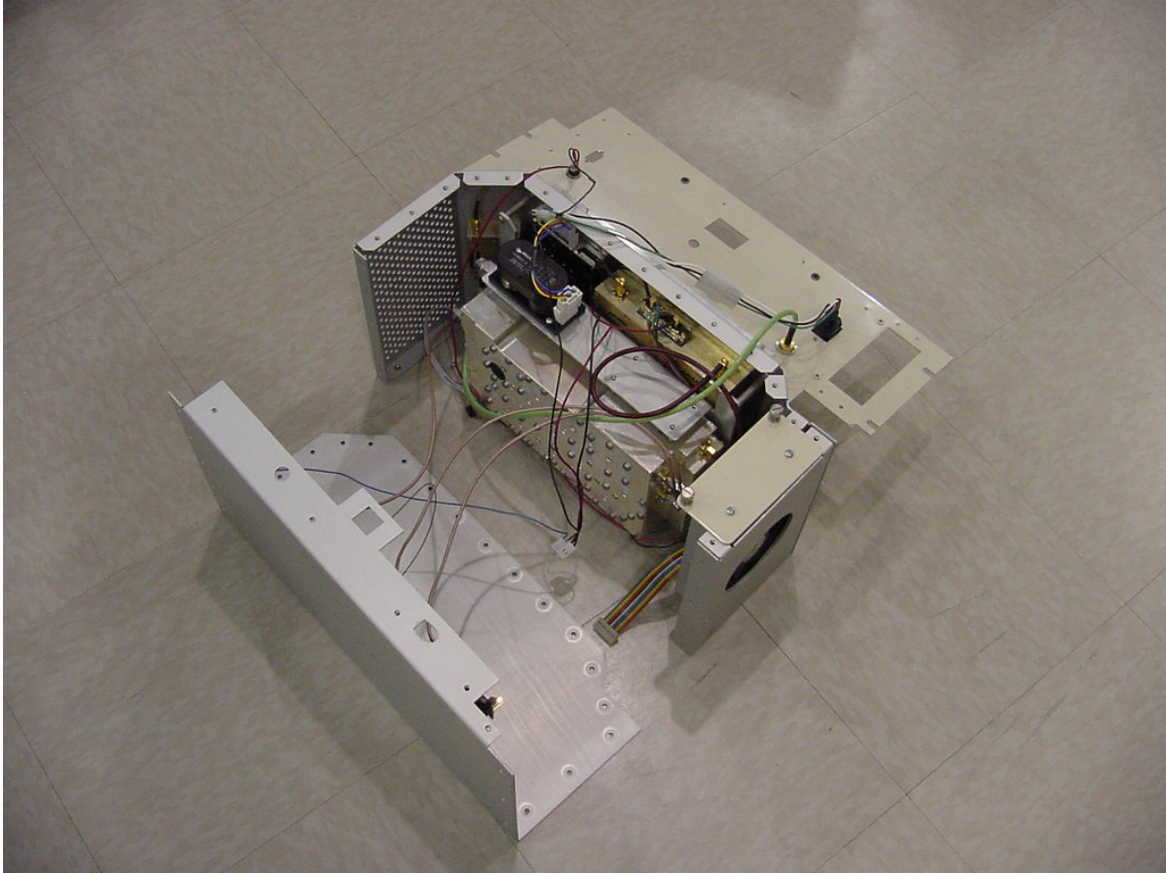
Digivance SCX - SMR Remote Unit Open View – Bottom Left
