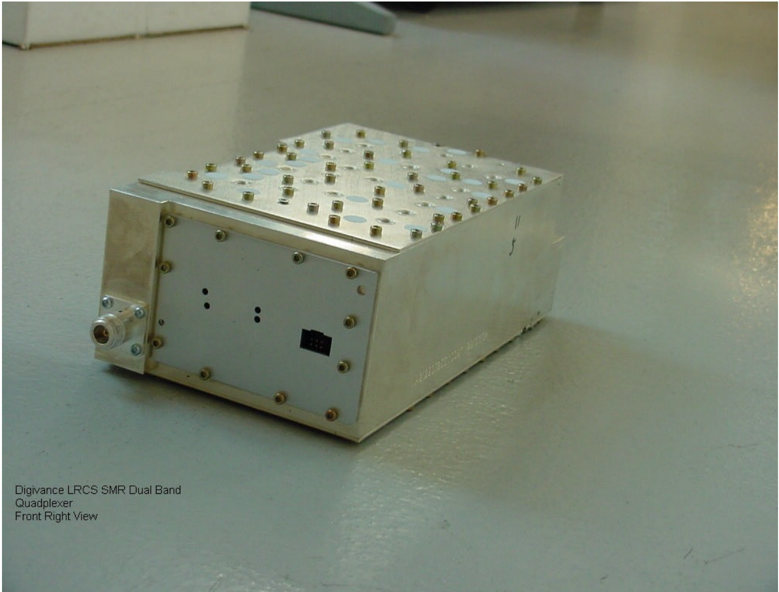
Digivance LRCS SMR Dual Band Quadplexer Front Right View
