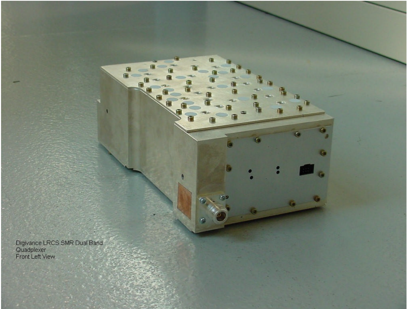
Digivance LRCS SMR Dual Band Quadplexer Front Left View
