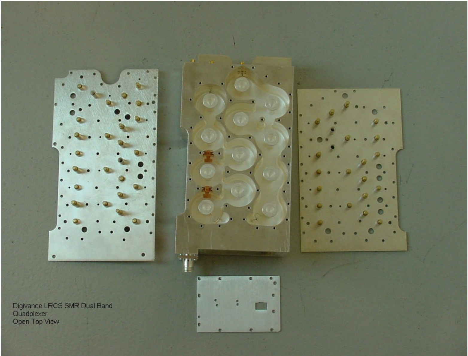
Digivance LRCS SMR Dual Band Quadplexer Open Top View
