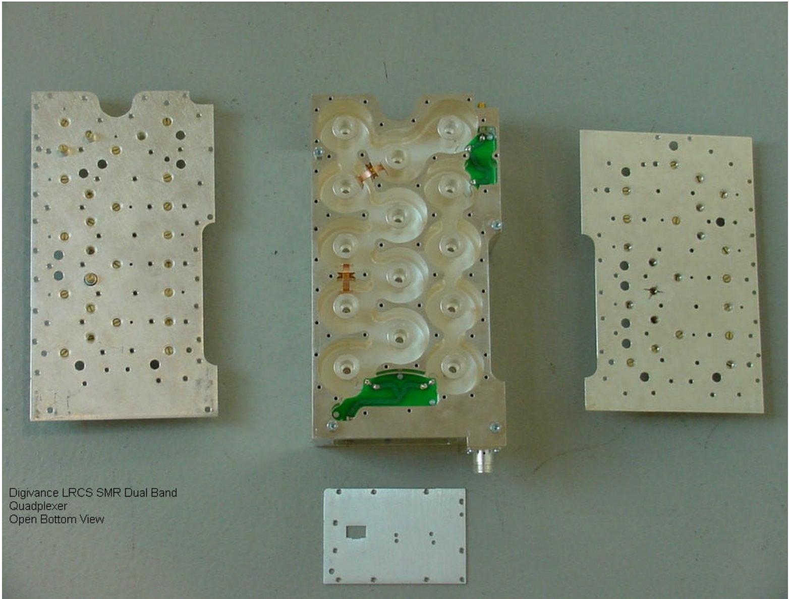
Digivance LRCS SMR Dual Band Quadplexer Open Bottom View
