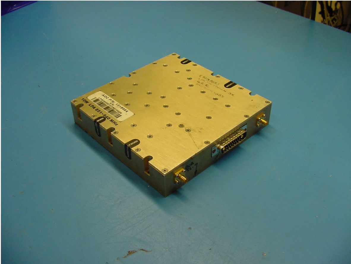
Bravo Tech SMR 800/900 Dual Band Linear Power Amplifier - 10 Watt Right View
