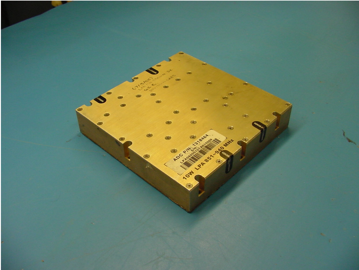
Bravo Tech SMR 800/900 Dual Band Linear Power Amplifier - 10 Watt Left View
