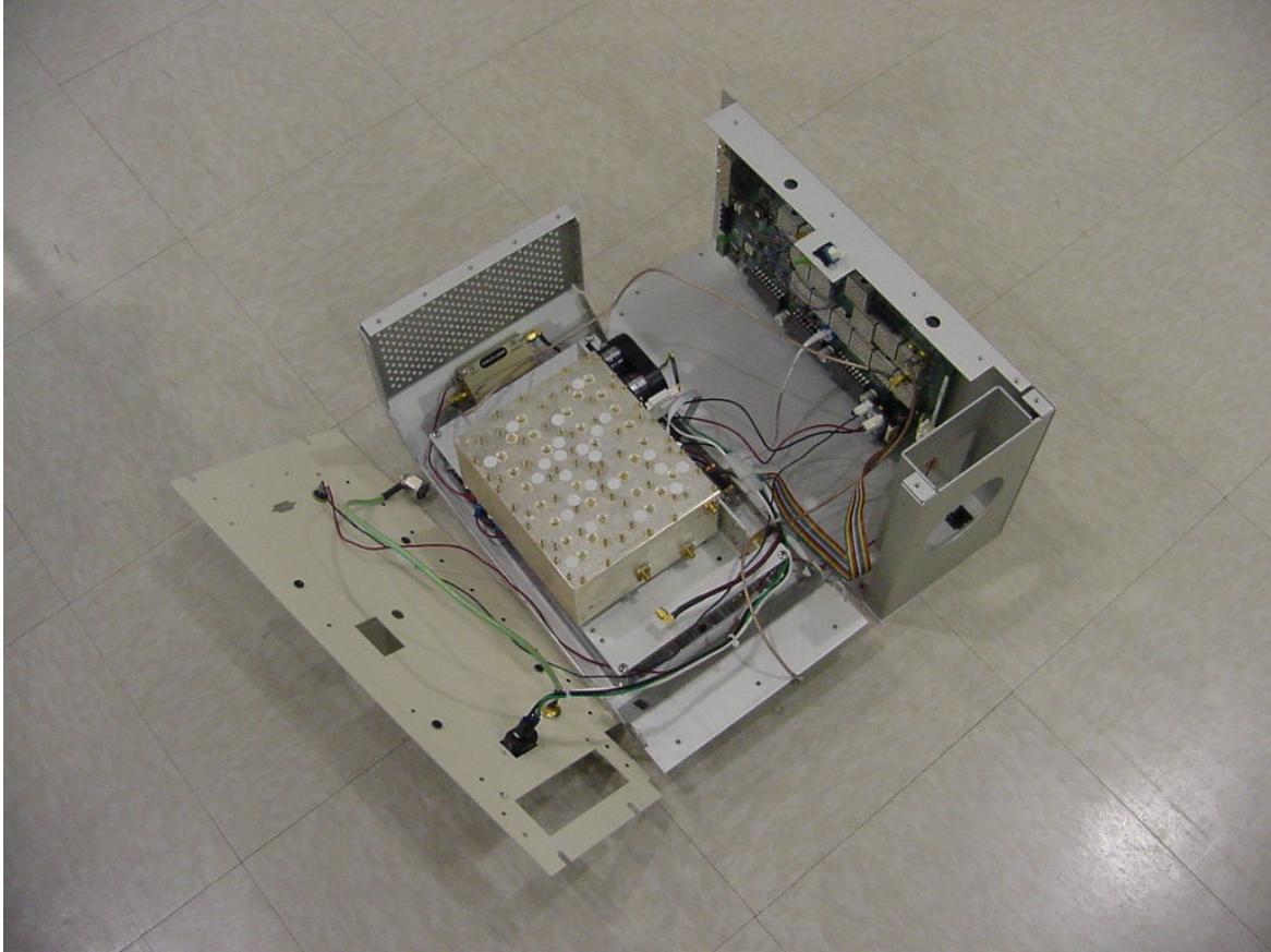
Digivance SCX - SMR Remote Unit Open View
