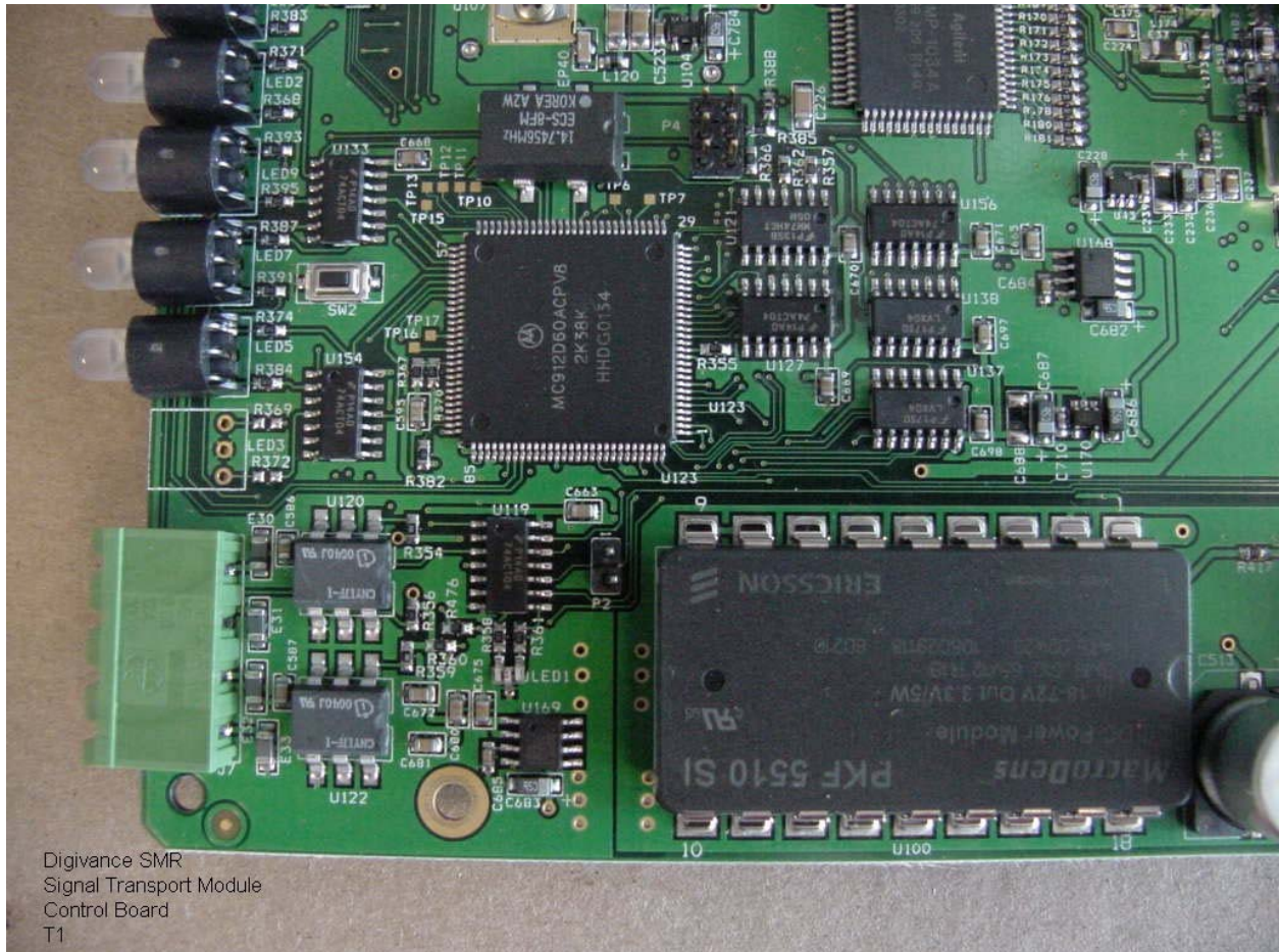
Digivance SMR Signal Transport Module Control Board Top View
