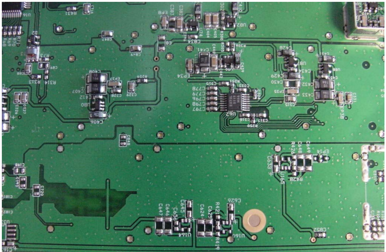
Digivance SMR Signal Transport Module Control Board B2
