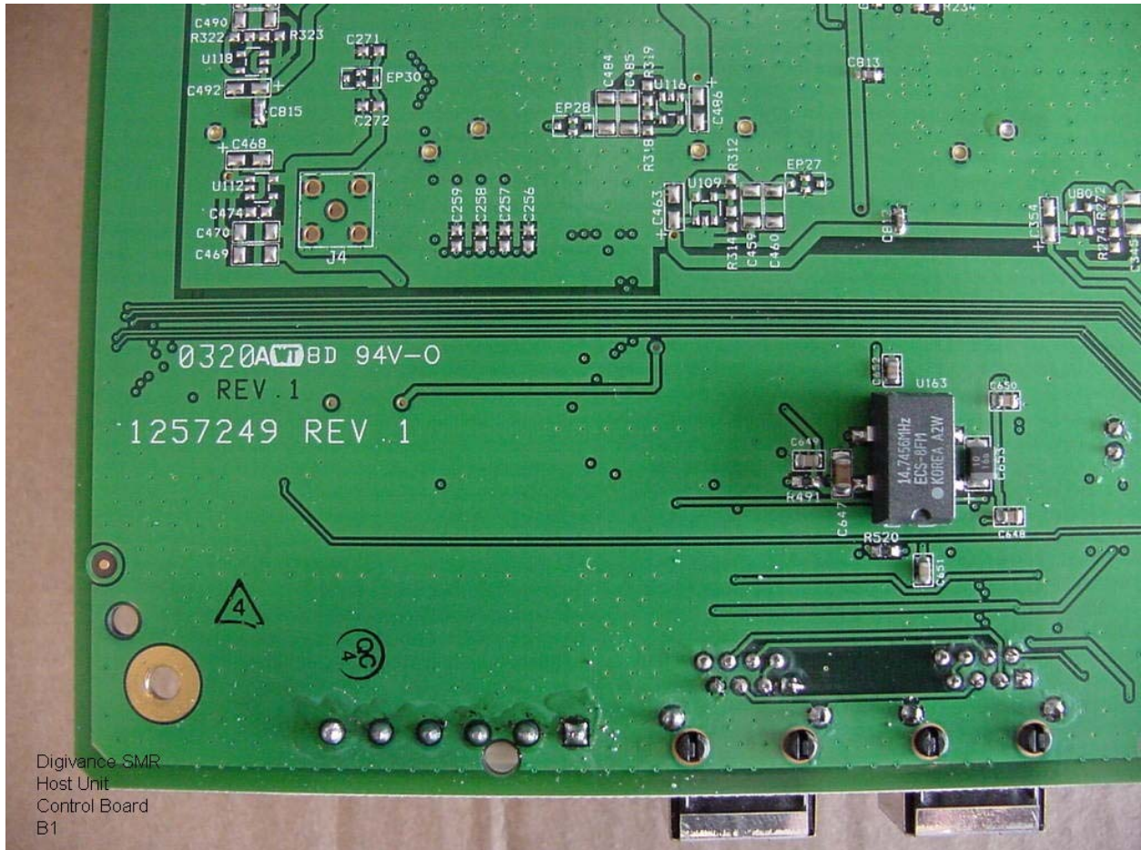
Digivance SMR Host Unit Control Board Bottom View
