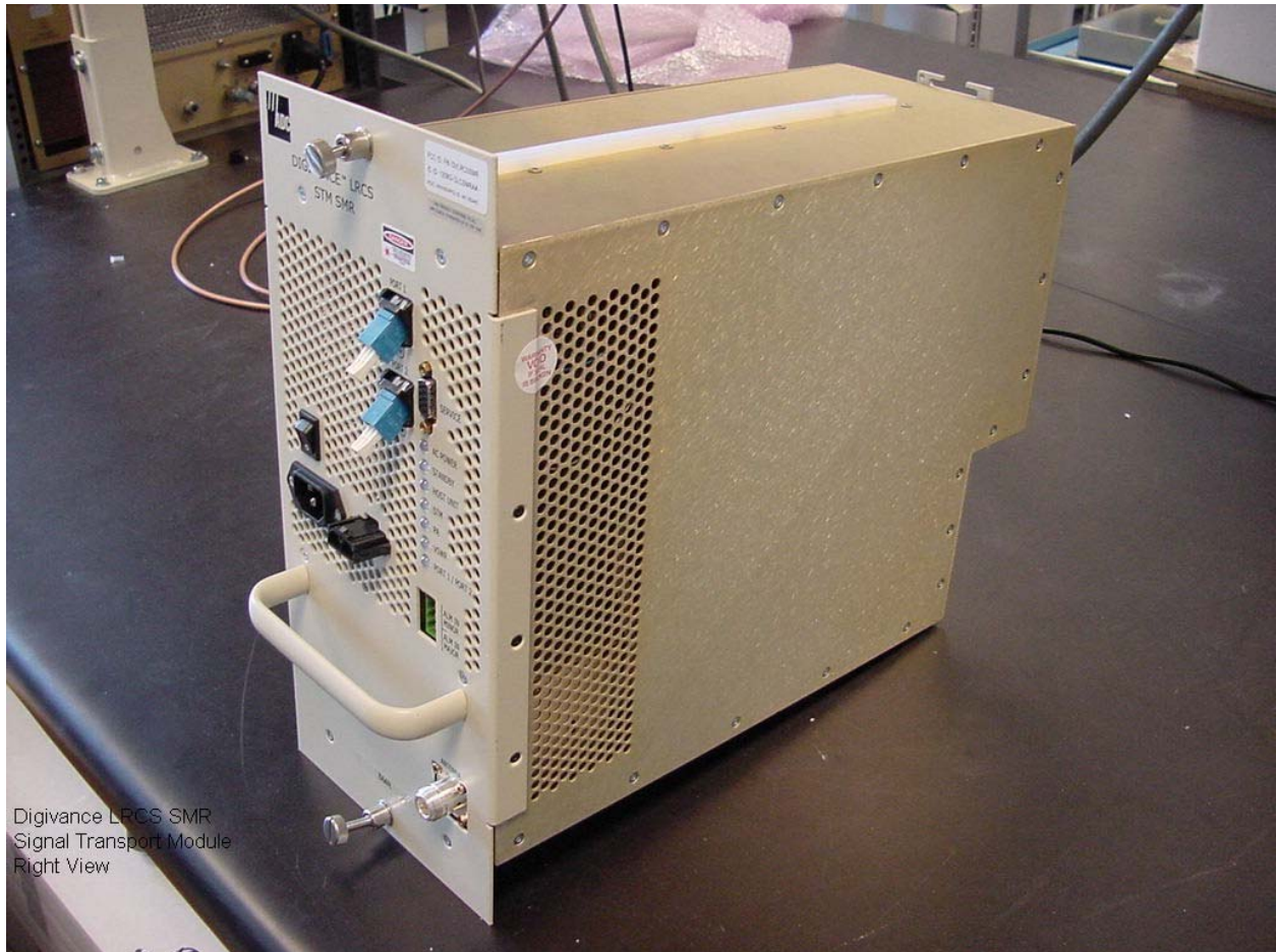
Digivance LRCS SMR Signal Transport Module Front View
