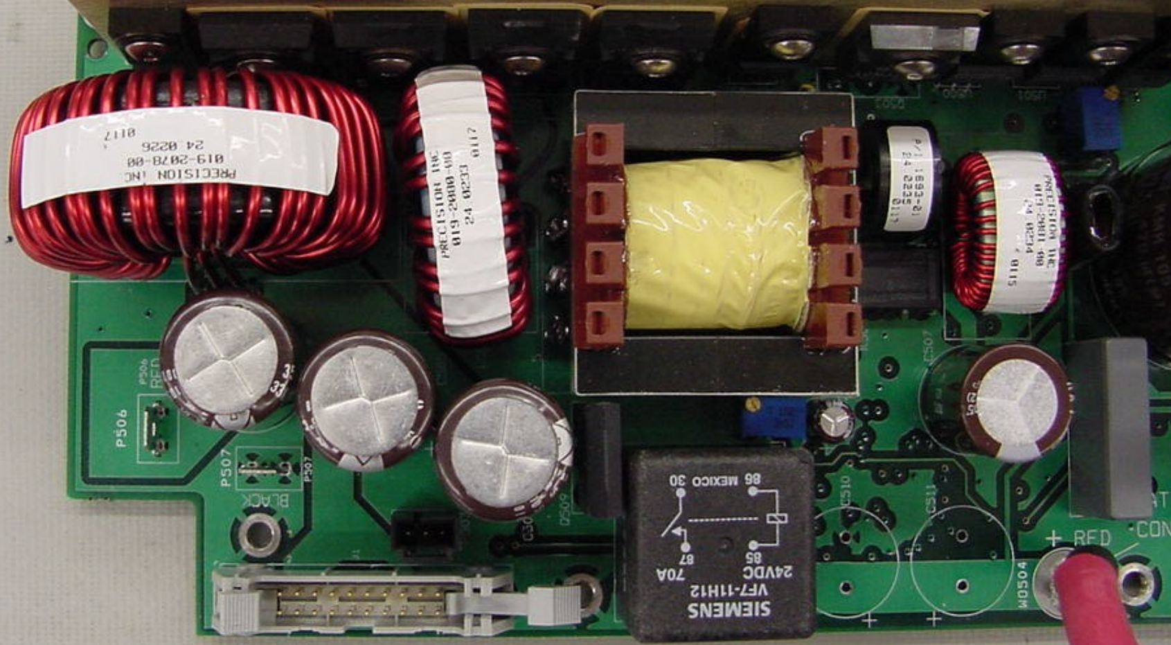
Digivance LRCS Power Supply Board Top View - Lower Left
