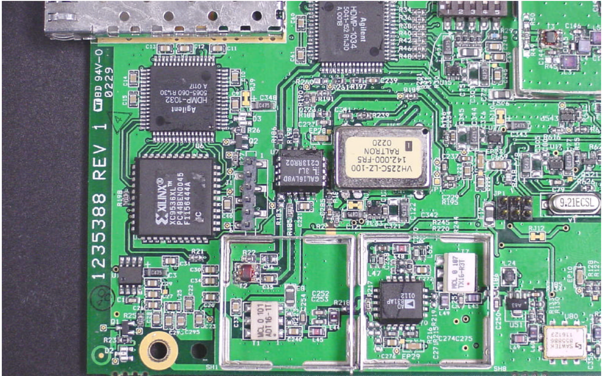
Digivance ICS SMR DRU Control Board - T1
