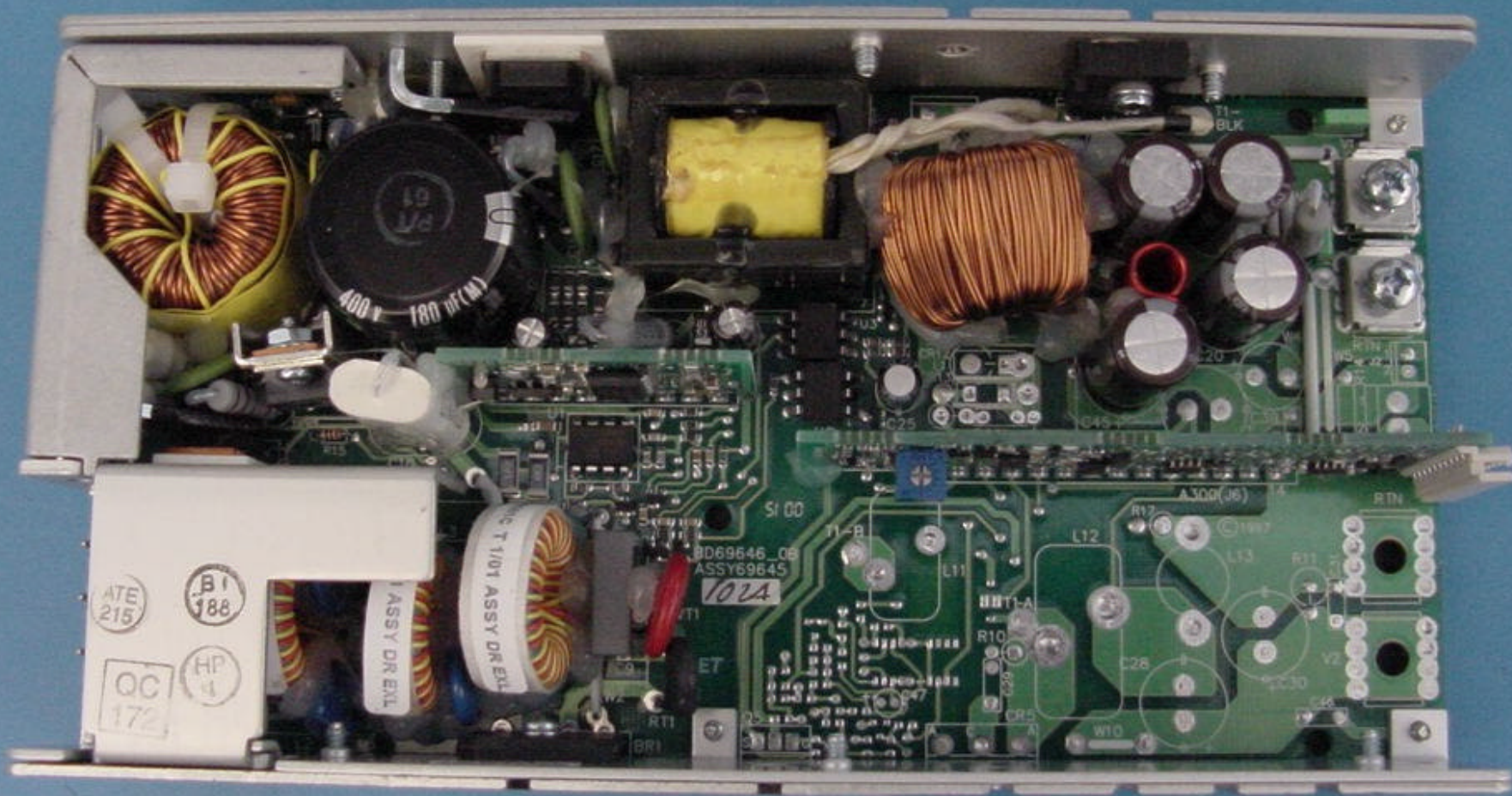
Digivance ICS Power Supply Top View
