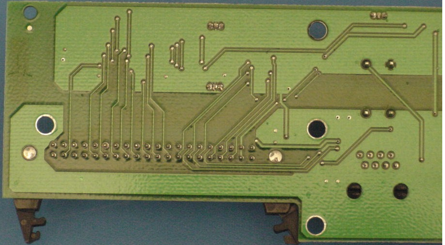
Digivance ICS SMR DHU Power Distribution Board - B1
