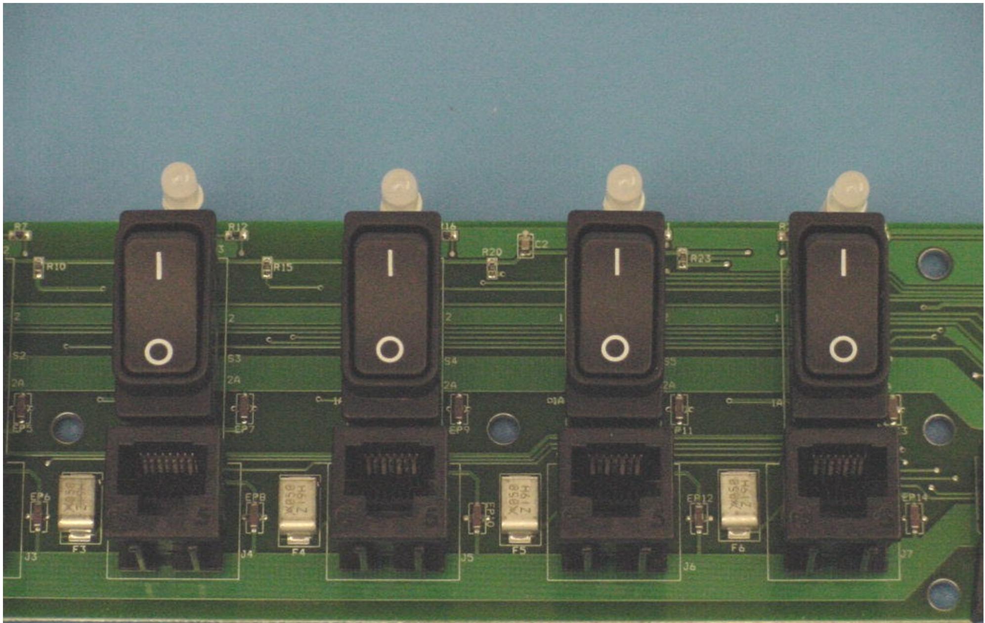
Digivance ICS SMR DHU Power Distribution Board - T2
