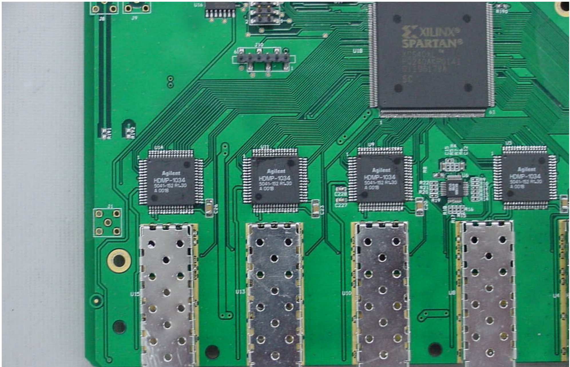
Digivance ICS SMR DHU Control Board - T1
