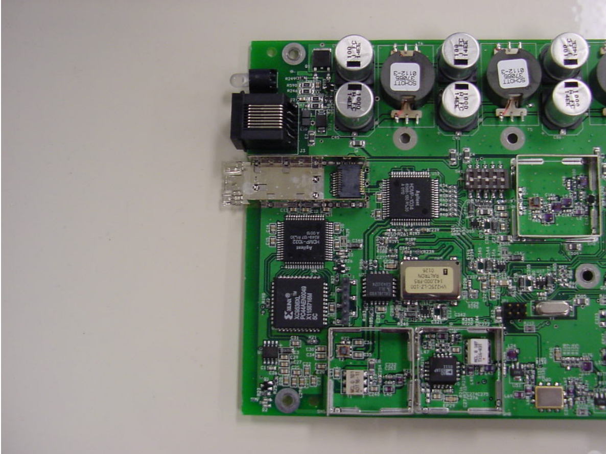
Digivance ICS 800 MHz Digital Remote Unit - PCB Top View - 1
