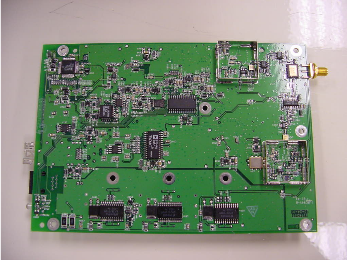
Digivance ICS 800 MHz Digital Remote Unit - PCB Bottom View
