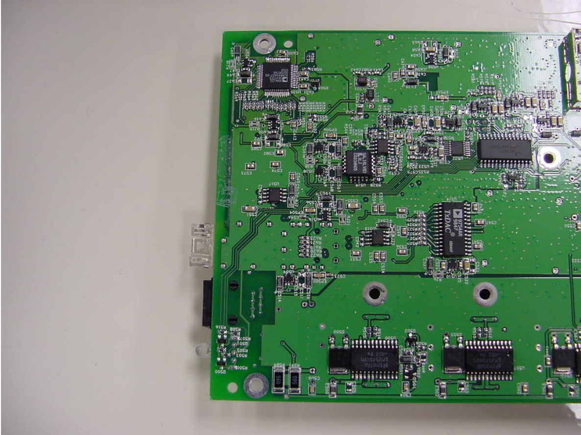
Digivance ICS 800 MHz Digital Remote Unit - PCB Bottom View - 1
