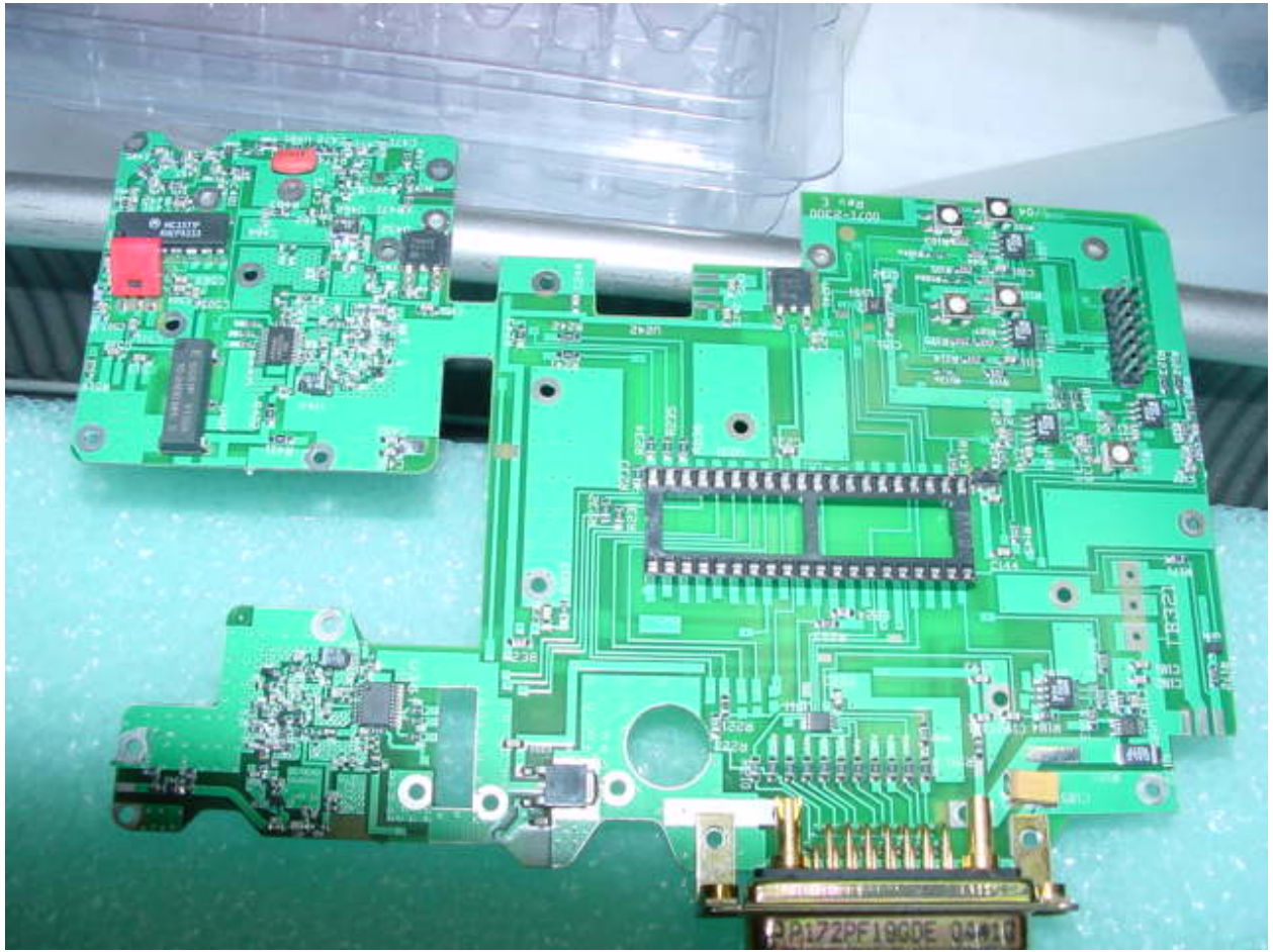
Broadband LPA Photos
