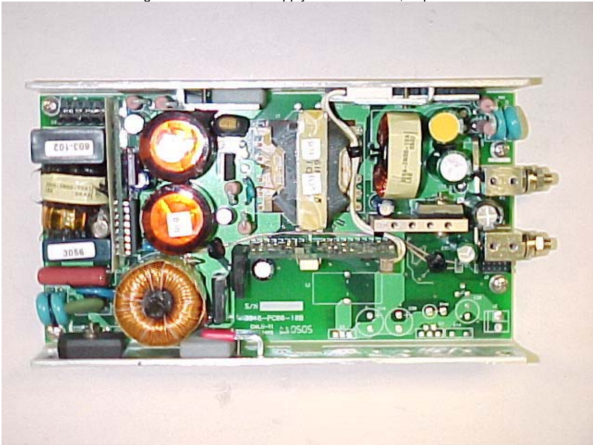
Digital Power - Power Supply - eFO306-1XX, Top View
