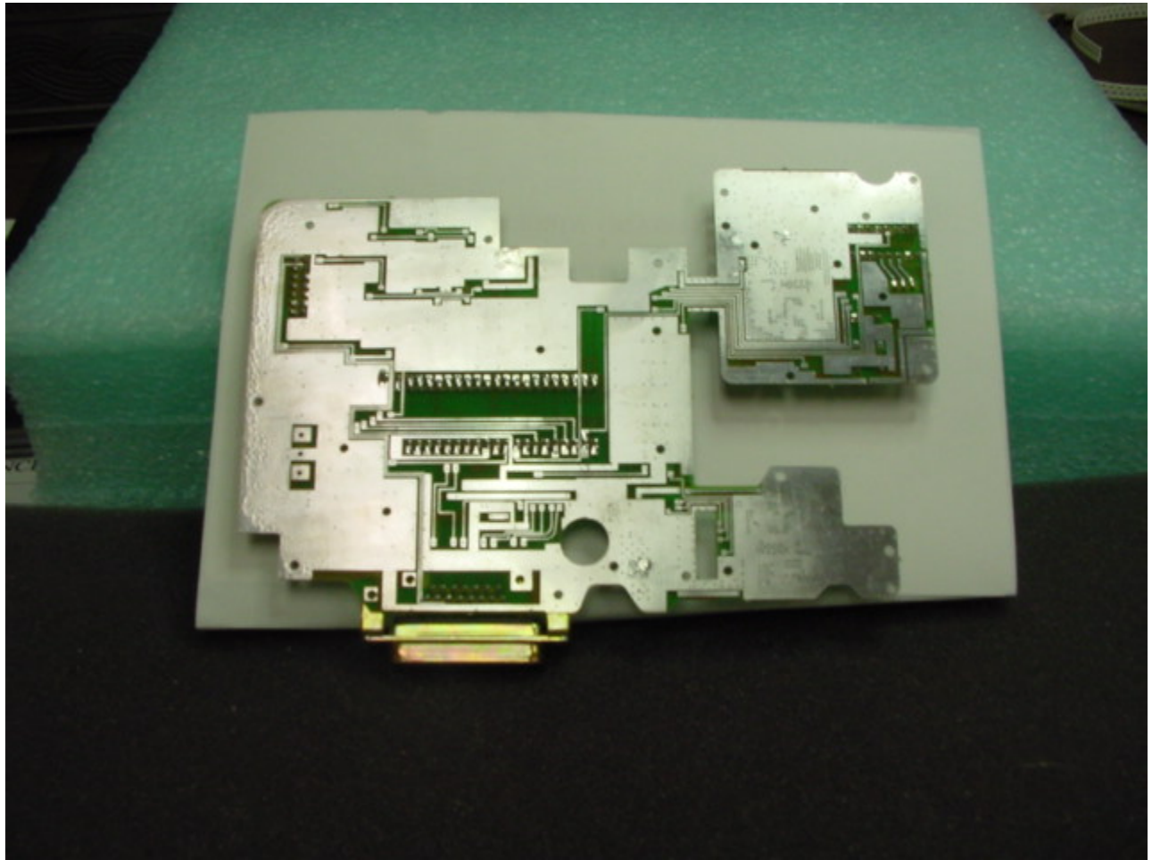
Broadband 20W LPA - Board 2 - Bottom View
