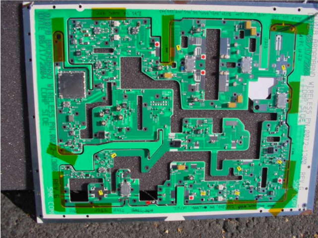
Broadband 20W LPA - 0072-1300 - Top View
