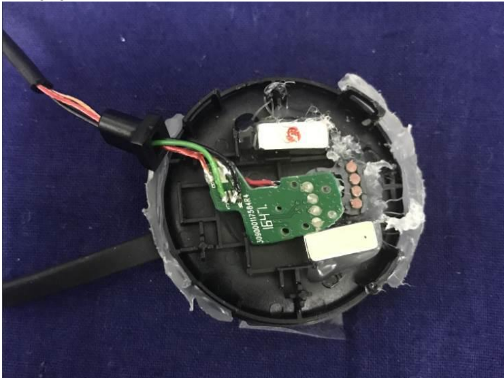
(6) Charging Cable Photo
