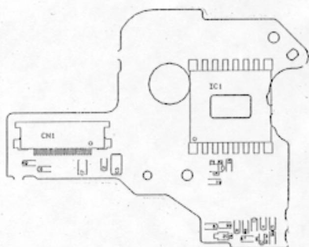
Lens Board
