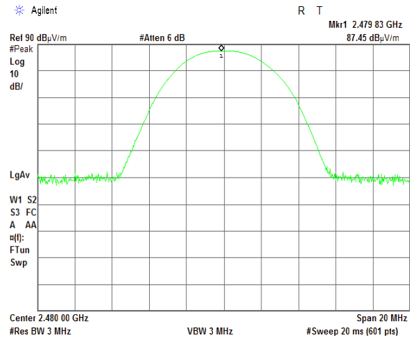
Horizontal antenna polarization
