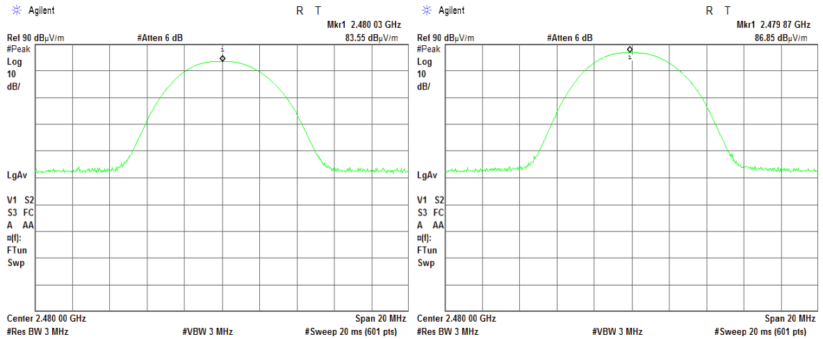
Vertical antenna polarization
