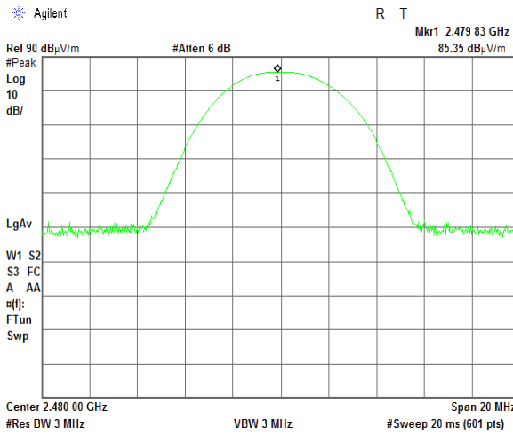
Vertical antenna polarization
