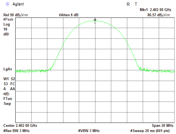
Horizontal antenna polarization
