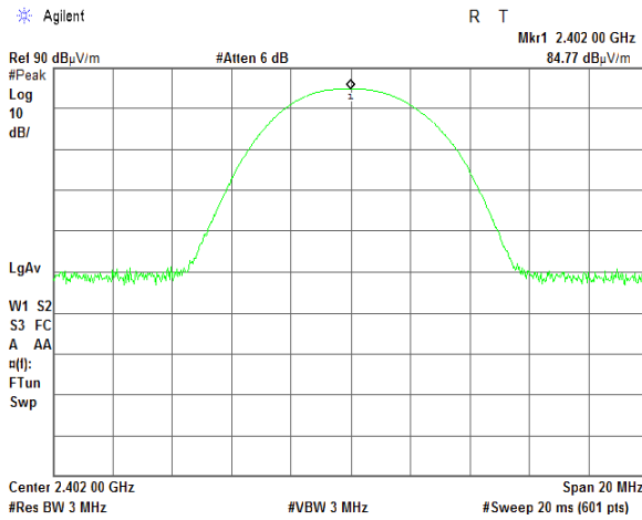
Vertical antenna polarization
