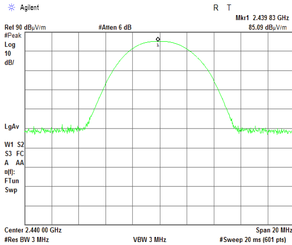
Vertical antenna polarization
