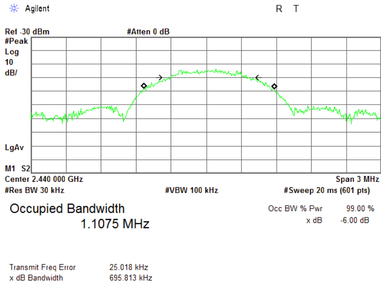
Plot 7.1.4 99% bandwidth test result at mid frequency
