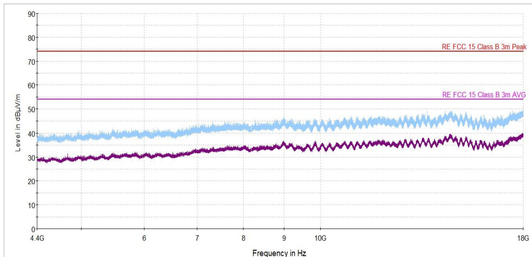
Plot 7.2.17 Radiated emission measurements from 4400 to 18000 MHz at the mid carrier frequency
