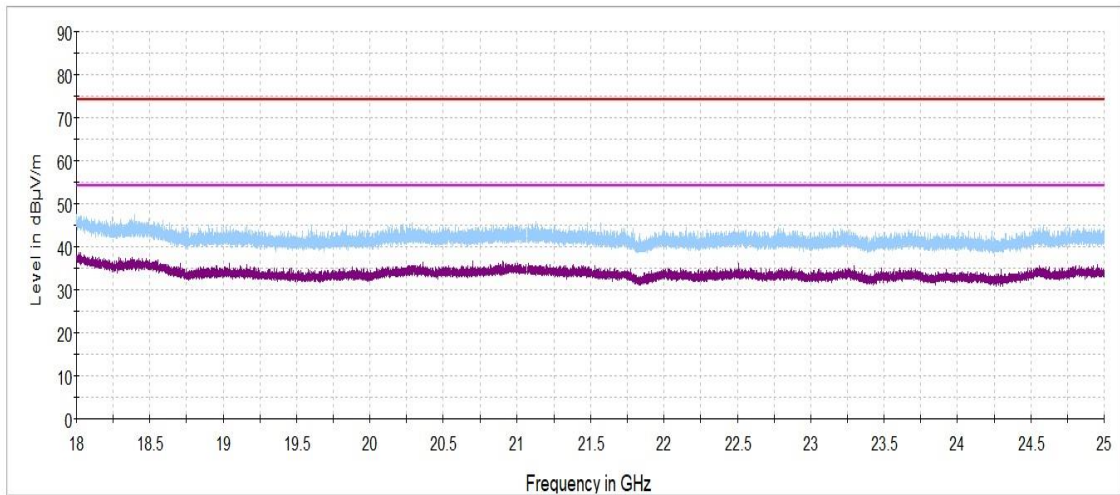
Plot 7.2.20 Radiated emission measurements from 18000 to 25000 MHz at the mid carrier frequency
