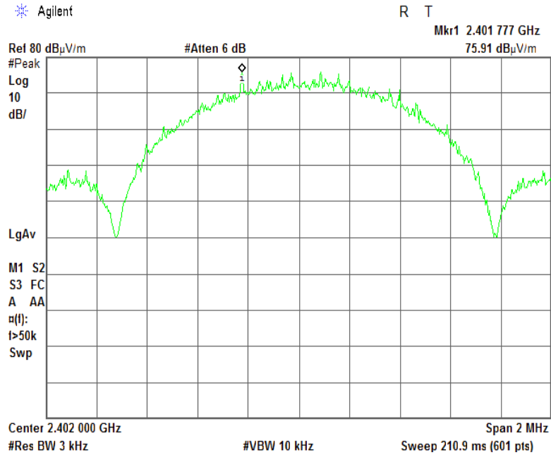
Plot 7.5.1 Peak spectral power density at low frequency
