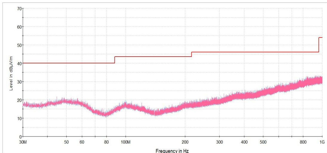
Plot 7.2.9 Radiated emission measurements from 30 to 1000 MHz at the high carrier frequency
