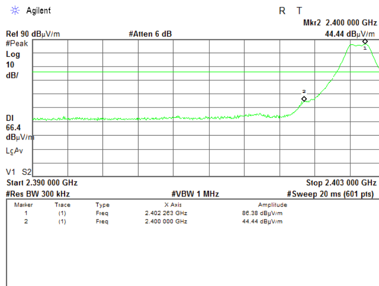
Plot 7.4.1 The highest band edge emission at low carrier frequency with hopping function disabled
