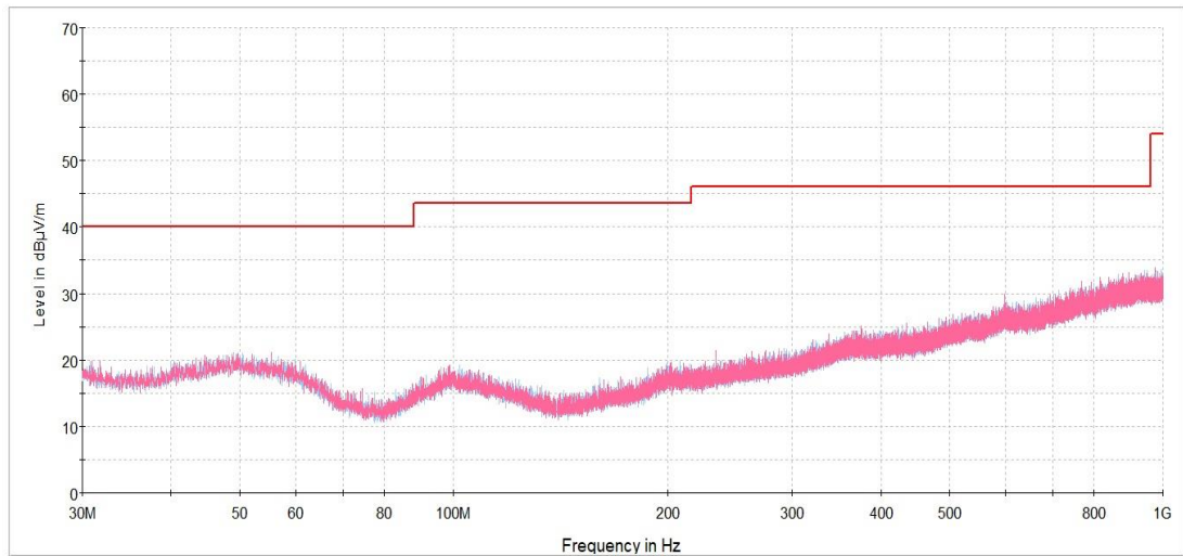
Plot 7.2.8 Radiated emission measurements from 30 to 1000 MHz at the mid carrier frequency
