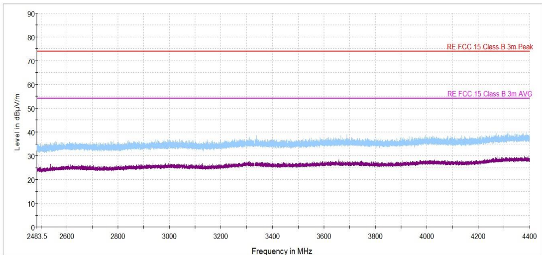
Plot 7.2.15 Radiated emission measurements from 2483.5 to 4400 MHz at the high carrier frequency
