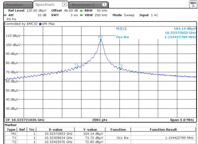
Figure 7.6-2: 99 % occupied bandwidth
