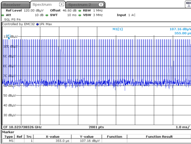
Figure 7.5-6: Pulse numbers per 10 ms
