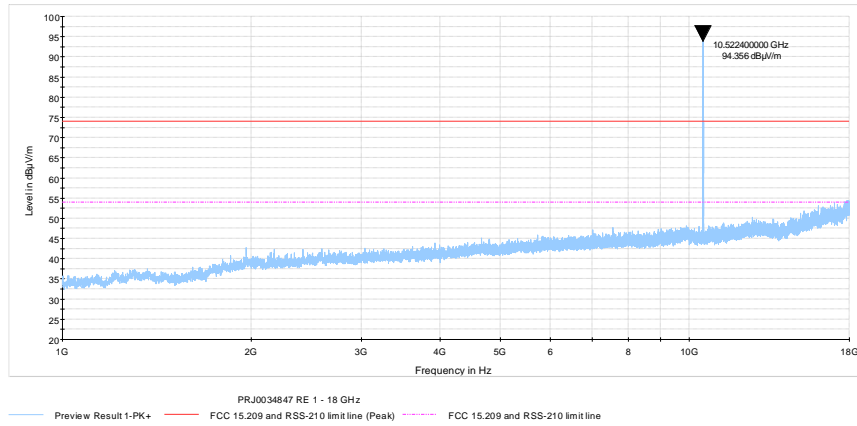
Figure 7-5-9: Field strength of spurious emissions within 1–18 GHz
