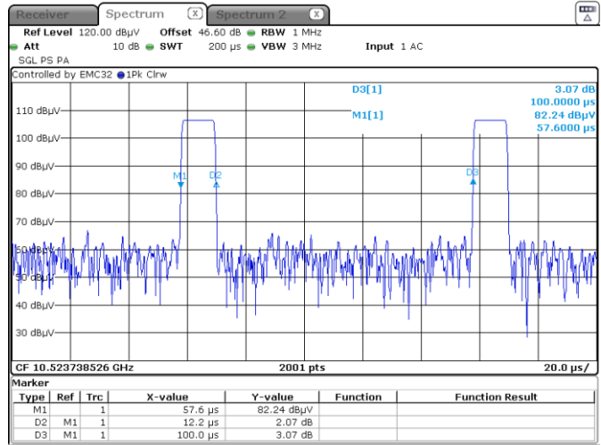
Figure 7.5-7: Pulse width
