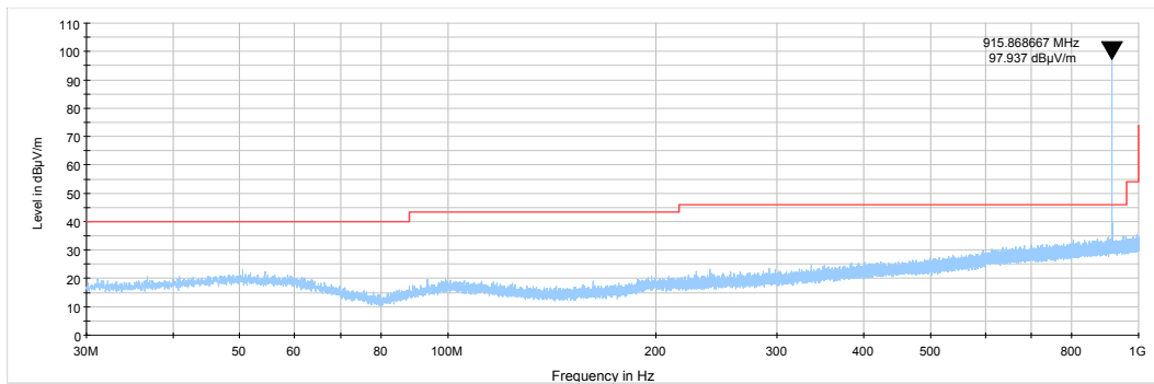
Plot 7.6.6 Radiated emission measurements from 30 to 1000 MHz at the high carrier frequency
