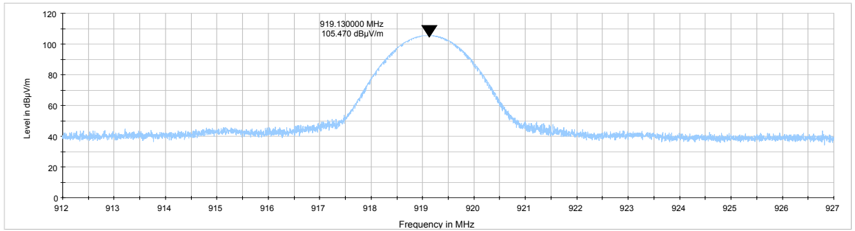
Plot 7.5.3 Field strength of carrier at high frequency
