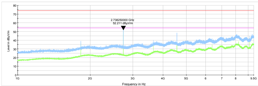
Plot 7.6.8 Radiated emission measurements from 1000 to 9500 MHz at the mid carrier frequency
