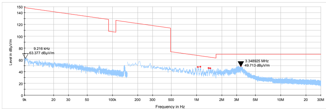
Plot 7.6.2 Radiated emission measurements from 9 kHz to 30 MHz at the mid carrier frequency
