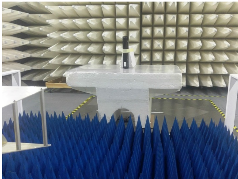
Photograph 8.1.2 Setup for radiated emission measurements above 1000 MHz
