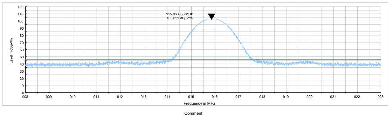
Plot 7.5.2 Field strength of carrier at mid frequency
