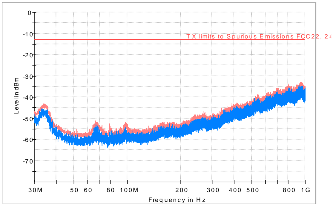
— PK+_MAXH — PK+_CLRWR — TX limits to Spurious Emissions FCC22, 24
