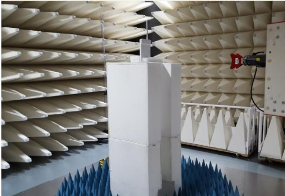
Figure C7. Radiated Emission test setup 3
