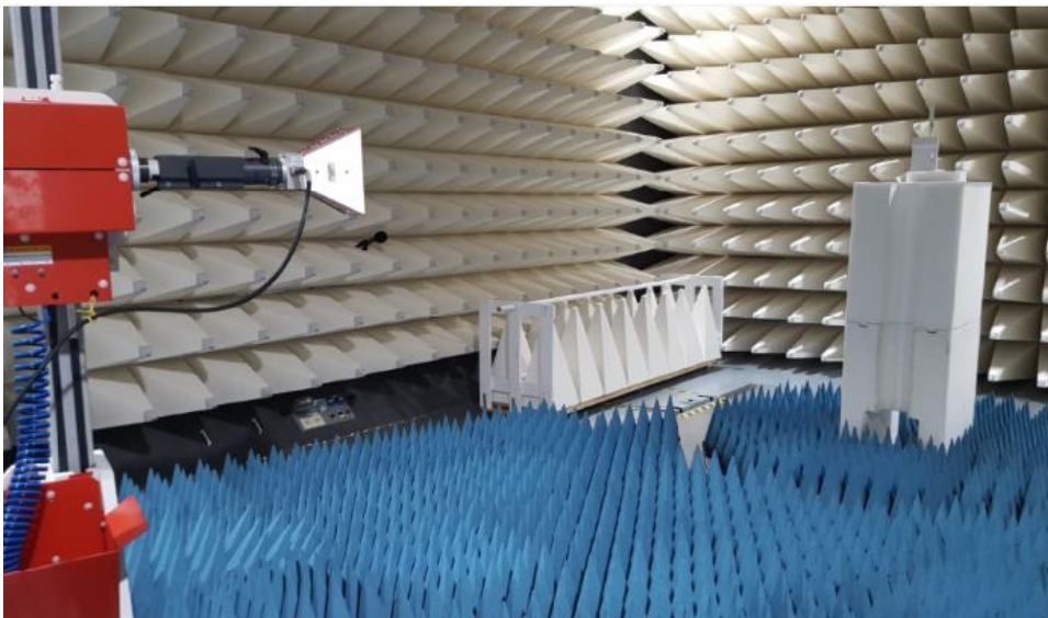
Figure C6. Radiated Emission test setup 2
