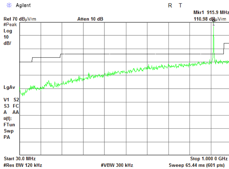
Plot 7.2.4 Radiated emission measurements from 30 to 1000 MHz at the high carrier frequency
