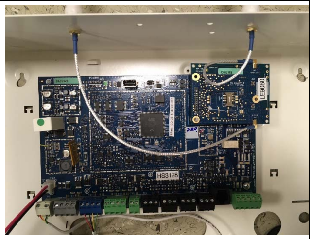
Host - Cover-off View 2
