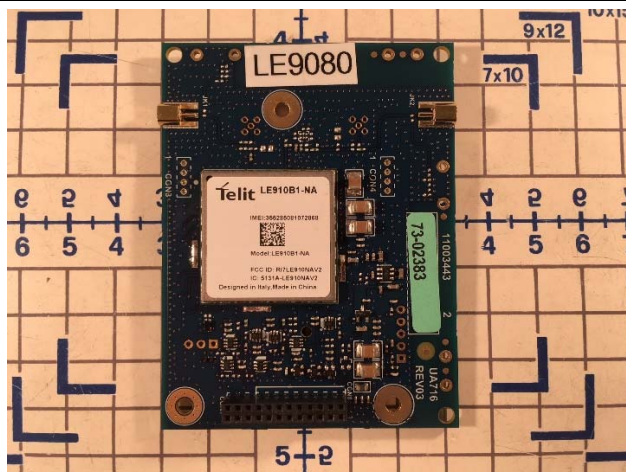
Module - Top View
