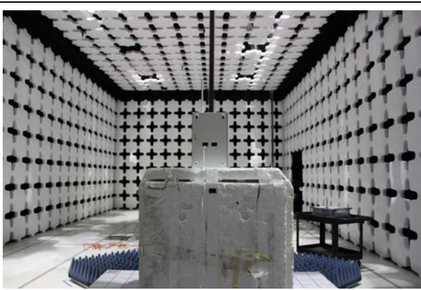
Spurious Emission Above 1GHz-Rear View
