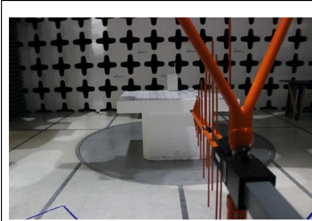
Spurious Emission Above 1GHz-Front View
