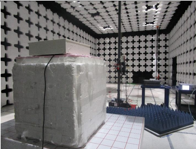
Spurious Emission Above 1GHz-Rear View
